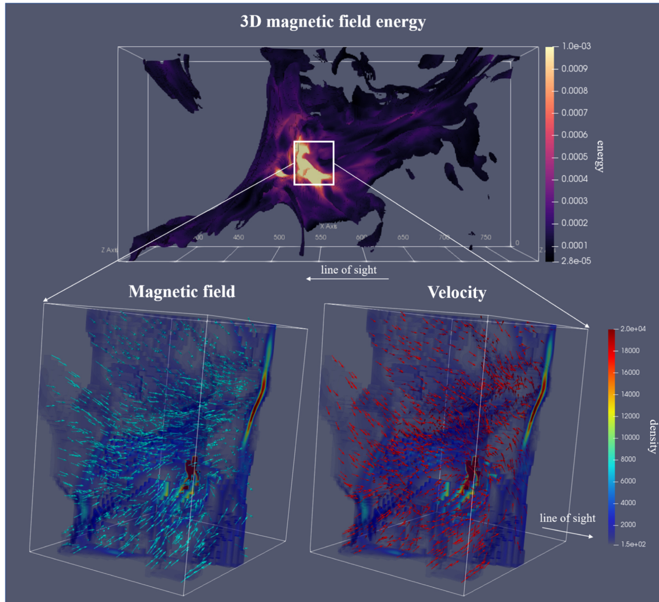
Figure 22. from Velocity Gradient in the Presence of Self-gravity: Identifying Gravity-induced Inflow and Determining Collapsing Stage null 2020 APJ 897 123 doi:10.3847/1538-4357/ab9948 https://dx.doi.org/10.3847/1538-4357/ab9948 © 2020. The American Astronomical Society. All rights reserved.
