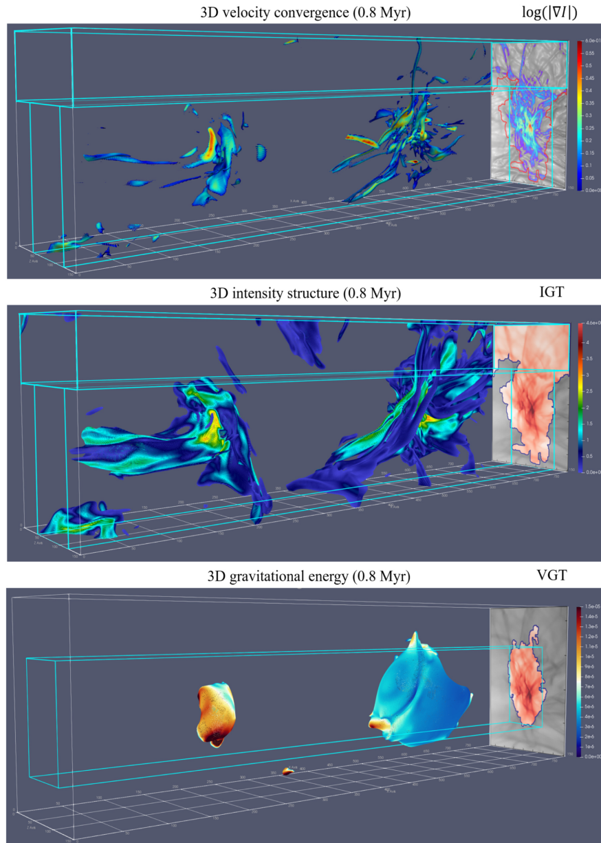
Figure 21. from Velocity Gradient in the Presence of Self-gravity: Identifying Gravity-induced Inflow and Determining Collapsing Stage null 2020 APJ 897 123 doi:10.3847/1538-4357/ab9948 https://dx.doi.org/10.3847/1538-4357/ab9948 © 2020. The American Astronomical Society. All rights reserved.
