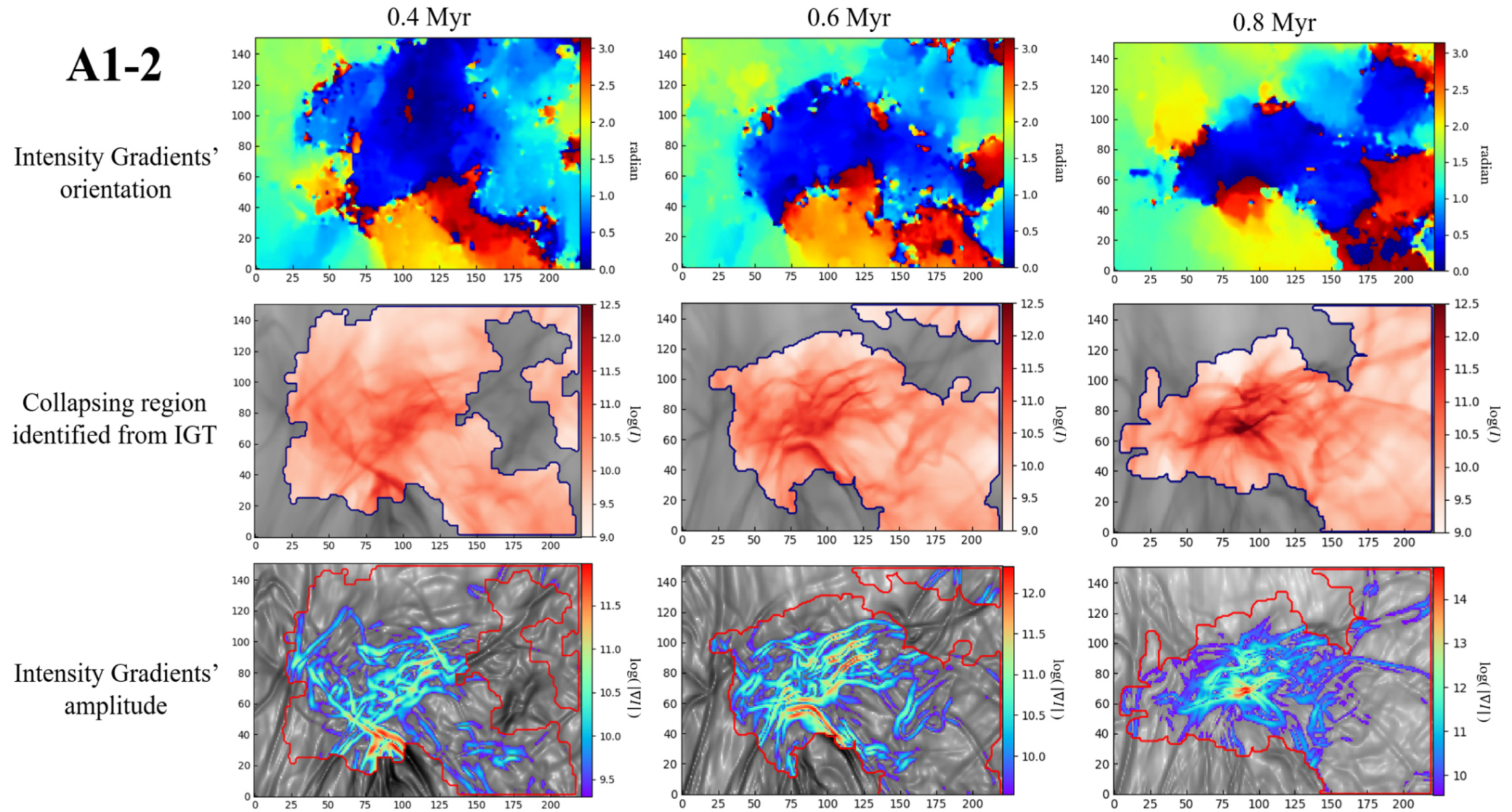
Figure 20. from Velocity Gradient in the Presence of Self-gravity: Identifying Gravity-induced Inflow and Determining Collapsing Stage null 2020 APJ 897 123 doi:10.3847/1538-4357/ab9948 https://dx.doi.org/10.3847/1538-4357/ab9948 © 2020. The American Astronomical Society. All rights reserved.
