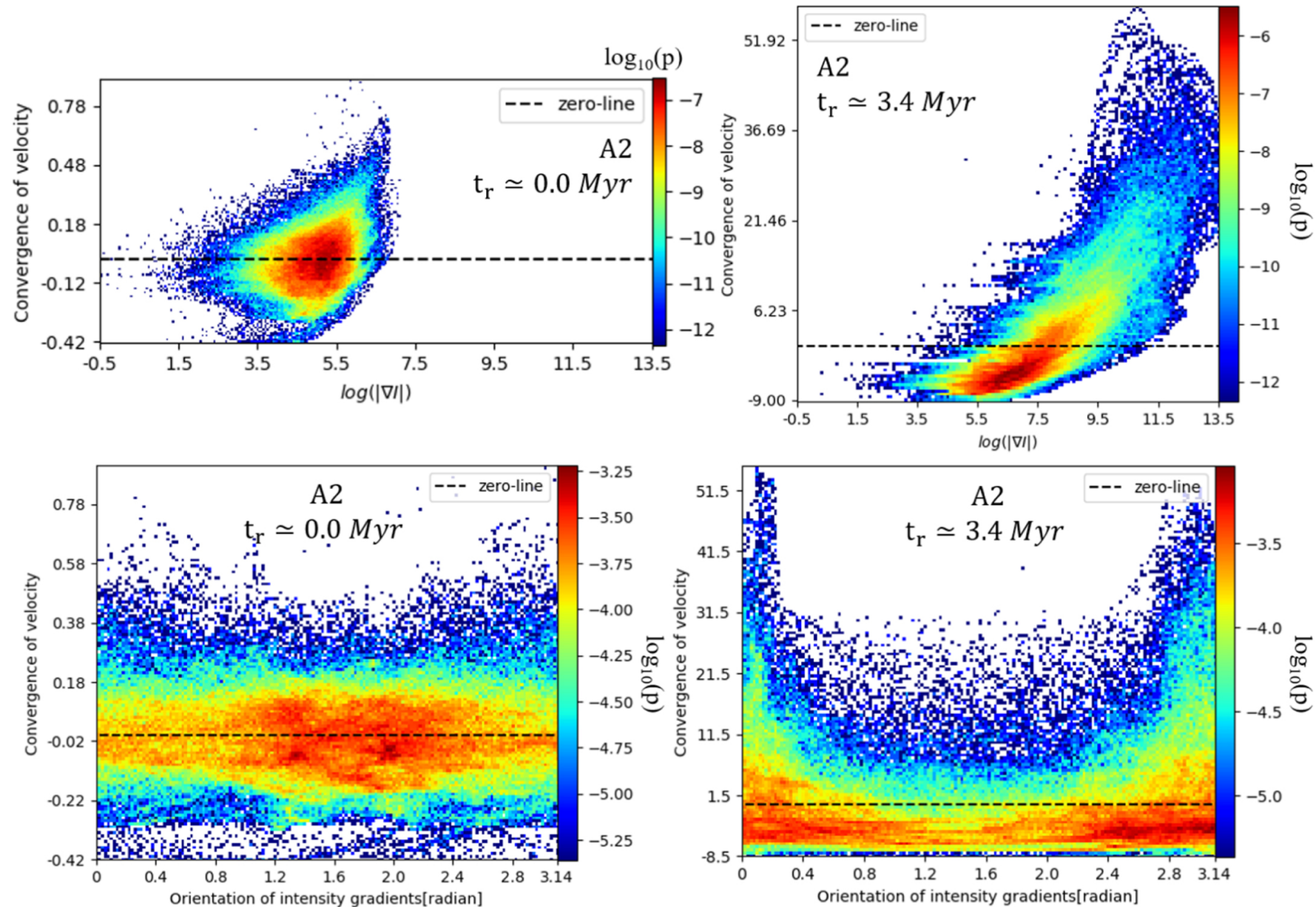
Figure 19. from Velocity Gradient in the Presence of Self-gravity: Identifying Gravity-induced Inflow and Determining Collapsing Stage null 2020 APJ 897 123 doi:10.3847/1538-4357/ab9948 https://dx.doi.org/10.3847/1538-4357/ab9948 © 2020. The American Astronomical Society. All rights reserved.
