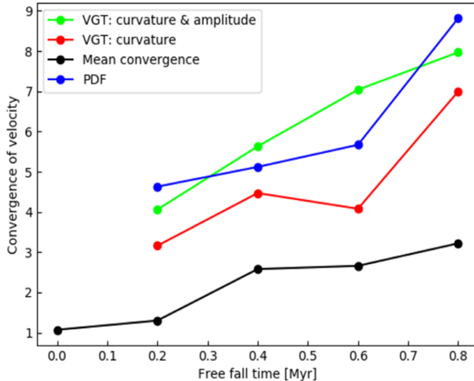
Figure 18. from Velocity Gradient in the Presence of Self-gravity: Identifying Gravity-induced Inflow and Determining Collapsing Stage null 2020 APJ 897 123 doi:10.3847/1538-4357/ab9948 https://dx.doi.org/10.3847/1538-4357/ab9948 © 2020. The American Astronomical Society. All rights reserved.
