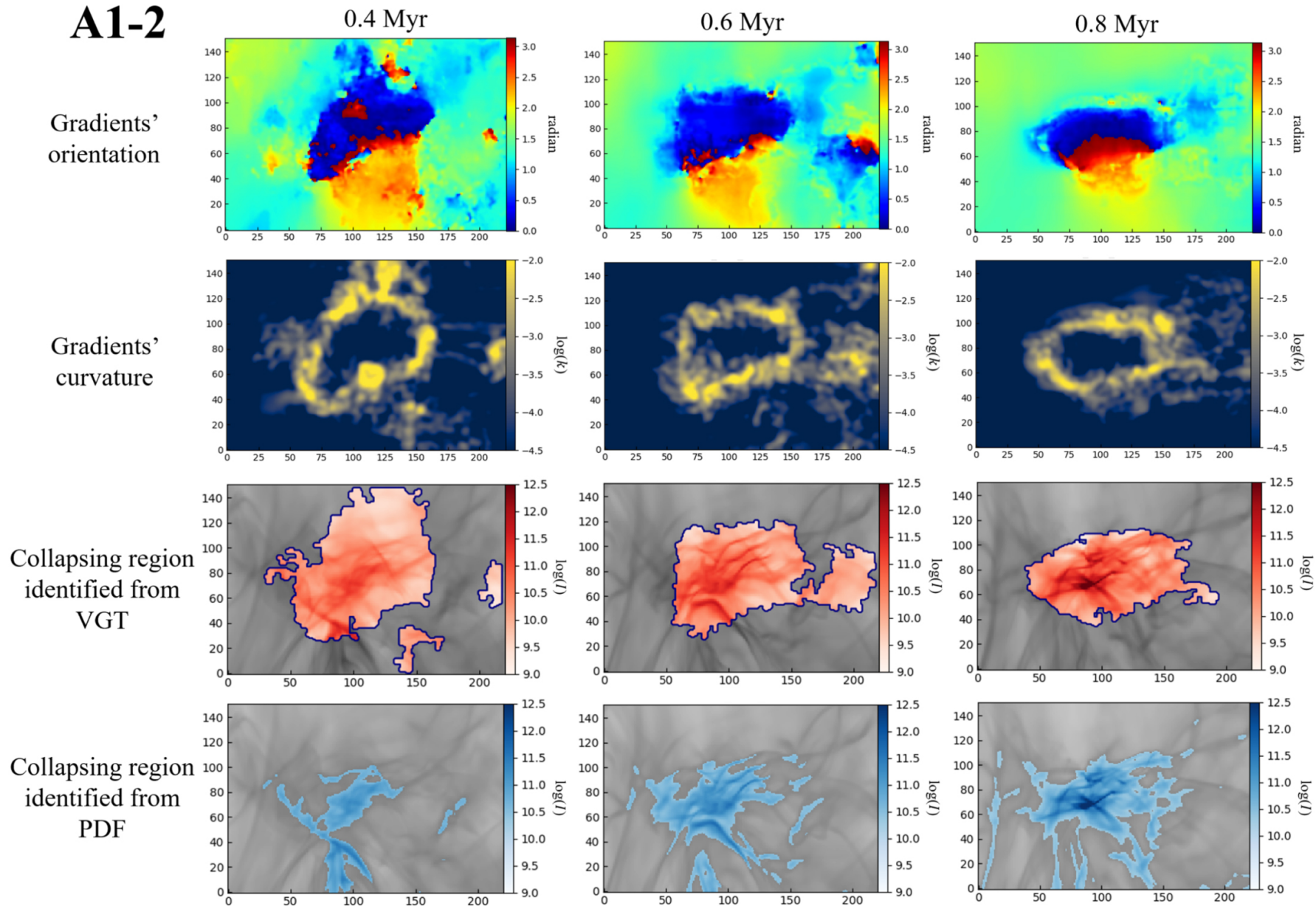
Figure 15. from Velocity Gradient in the Presence of Self-gravity: Identifying Gravity-induced Inflow and Determining Collapsing Stage null 2020 APJ 897 123 doi:10.3847/1538-4357/ab9948 https://dx.doi.org/10.3847/1538-4357/ab9948 © 2020. The American Astronomical Society. All rights reserved.
