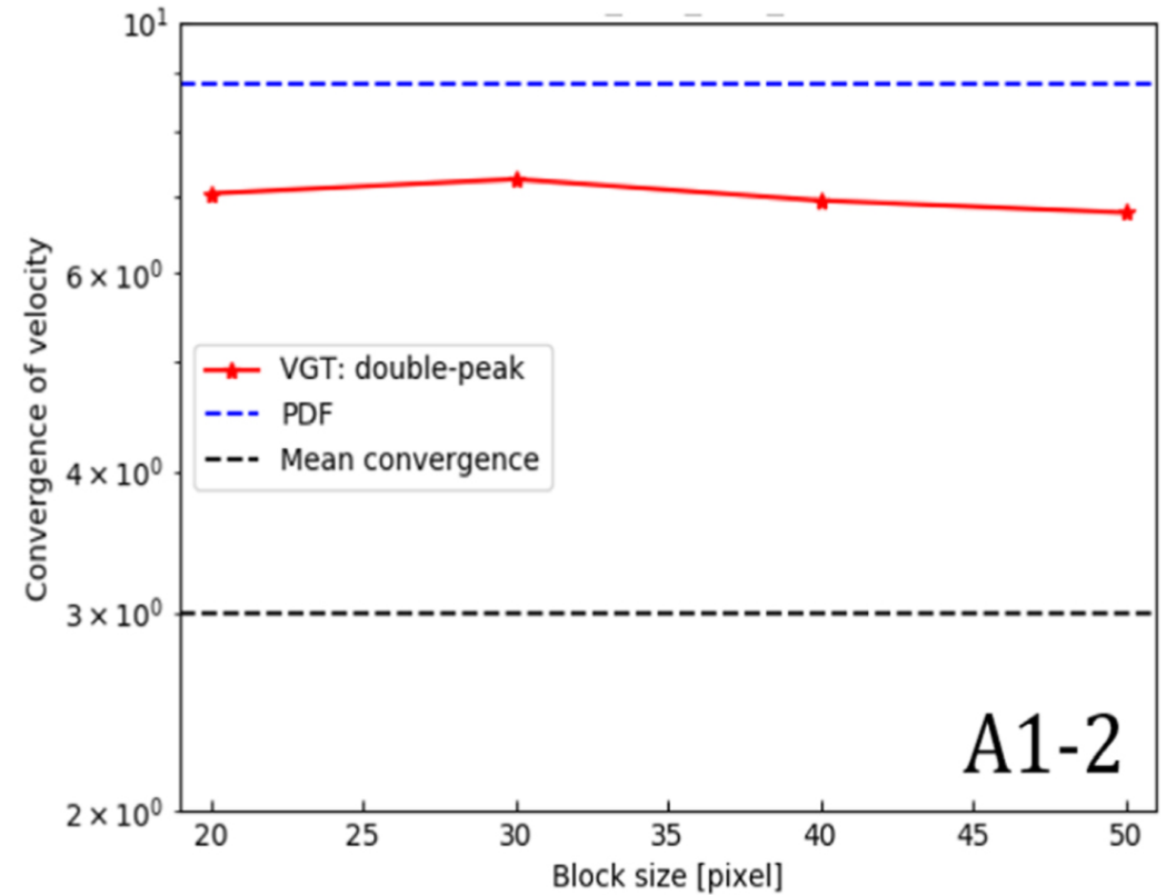
Figure 14. from Velocity Gradient in the Presence of Self-gravity: Identifying Gravity-induced Inflow and Determining Collapsing Stage null 2020 APJ 897 123 doi:10.3847/1538-4357/ab9948 https://dx.doi.org/10.3847/1538-4357/ab9948 © 2020. The American Astronomical Society. All rights reserved.
