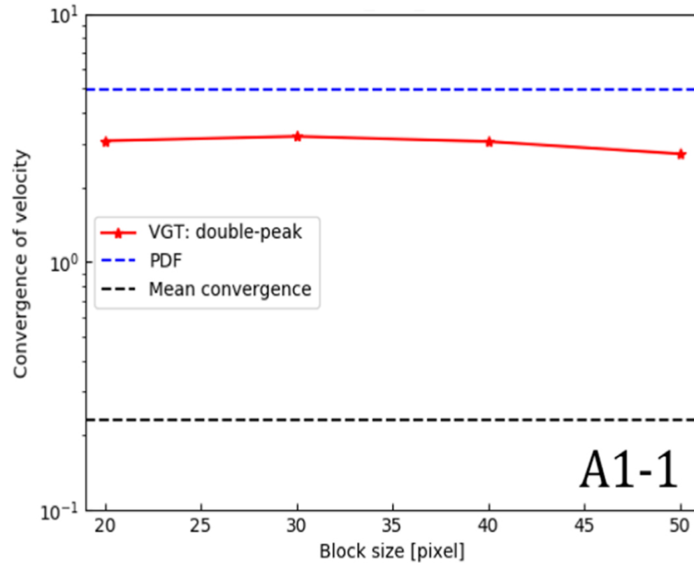
Figure 14. from Velocity Gradient in the Presence of Self-gravity: Identifying Gravity-induced Inflow and Determining Collapsing Stage null 2020 APJ 897 123 doi:10.3847/1538-4357/ab9948 https://dx.doi.org/10.3847/1538-4357/ab9948 © 2020. The American Astronomical Society. All rights reserved.
