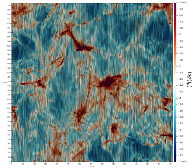
Figure 12. from Velocity Gradient in the Presence of Self-gravity: Identifying Gravity-induced Inflow and Determining Collapsing Stage null 2020 APJ 897 123 doi:10.3847/1538-4357/ab9948 https://dx.doi.org/10.3847/1538-4357/ab9948 © 2020. The American Astronomical Society. All rights reserved.
