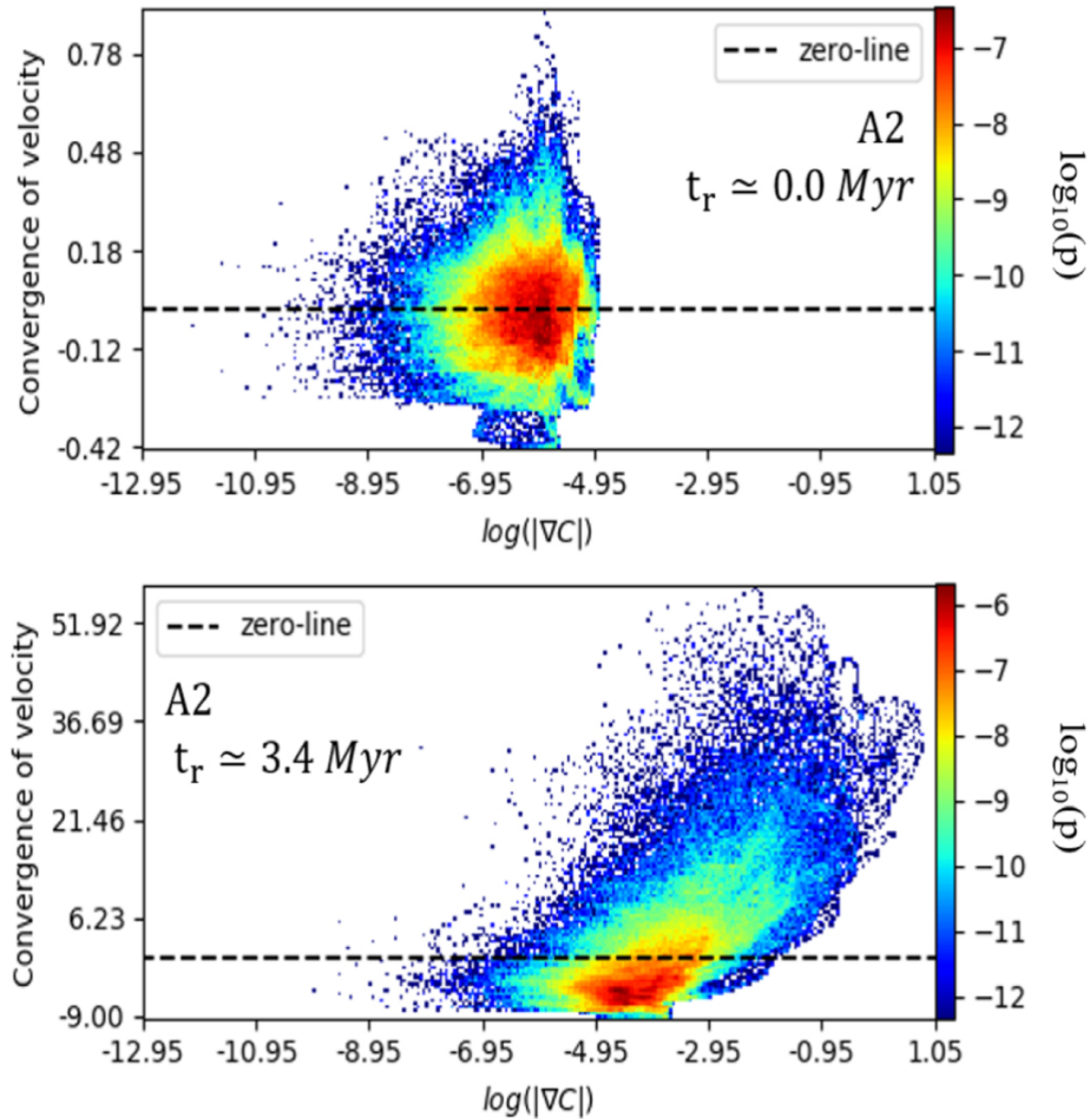
Figure 11. from Velocity Gradient in the Presence of Self-gravity: Identifying Gravity-induced Inflow and Determining Collapsing Stage null 2020 APJ 897 123 doi:10.3847/1538-4357/ab9948 https://dx.doi.org/10.3847/1538-4357/ab9948 © 2020. The American Astronomical Society. All rights reserved.
