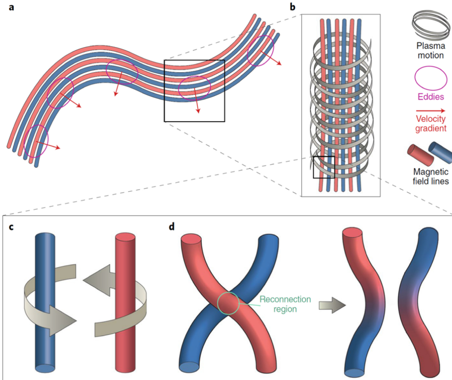
Figure 1. from Velocity Gradient in the Presence of Self-gravity: Identifying Gravity-induced Inflow and Determining Collapsing Stage null 2020 APJ 897 123 doi:10.3847/1538-4357/ab9948 https://dx.doi.org/10.3847/1538-4357/ab9948 © 2020. The American Astronomical Society. All rights reserved.
