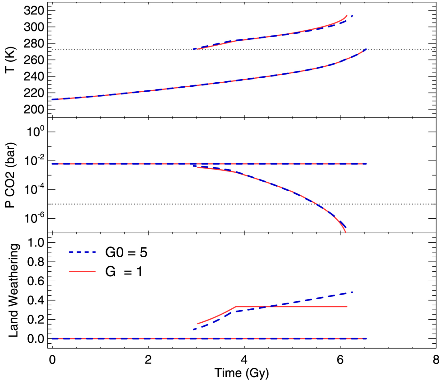
Figure 6. from The Effect of Seafloor Weathering on Planetary Habitability null 2020 APJ 896 96 doi:10.3847/1538-4357/ab94a4 https://dx.doi.org/10.3847/1538-4357/ab94a4 © 2020. The American Astronomical Society. All rights reserved.
