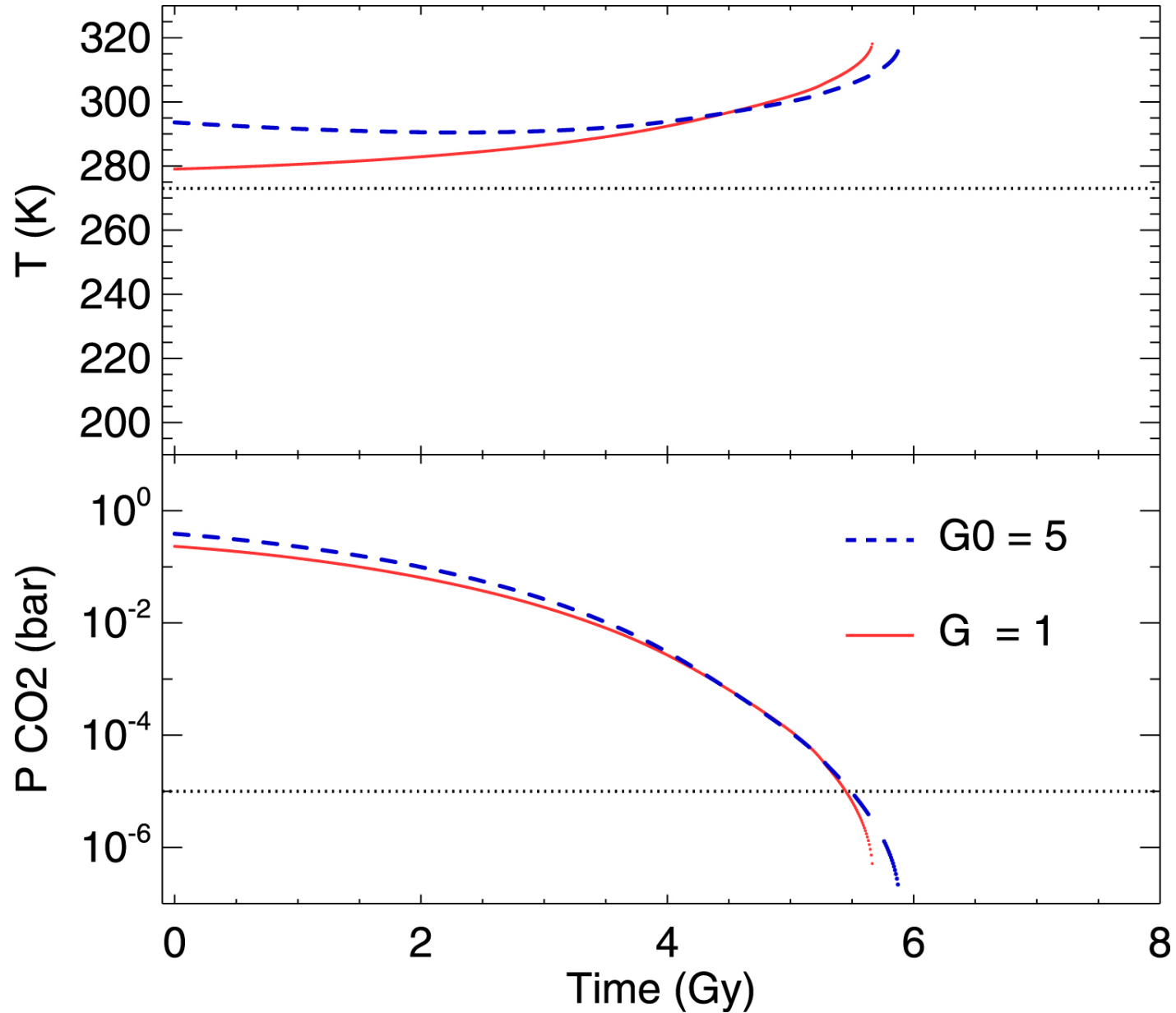
Figure 3. from The Effect of Seafloor Weathering on Planetary Habitability null 2020 APJ 896 96 doi:10.3847/1538-4357/ab94a4 https://dx.doi.org/10.3847/1538-4357/ab94a4 © 2020. The American Astronomical Society. All rights reserved.
