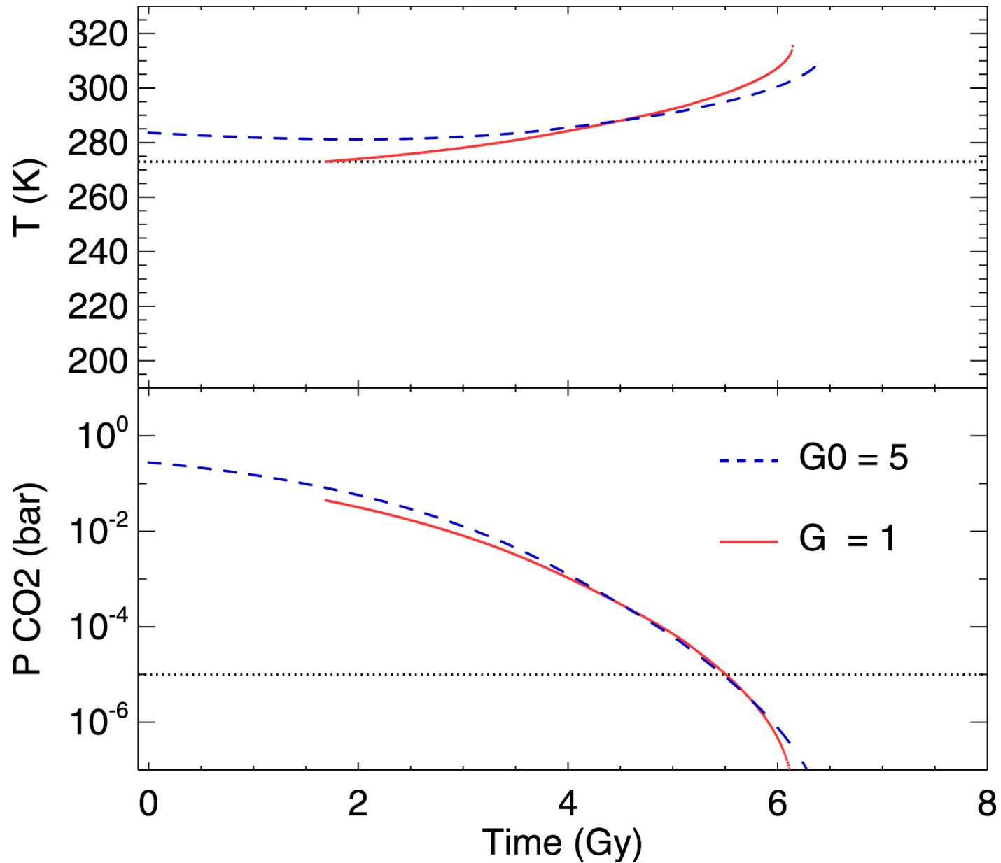
Figure 2. from The Effect of Seafloor Weathering on Planetary Habitability null 2020 APJ 896 96 doi:10.3847/1538-4357/ab94a4 https://dx.doi.org/10.3847/1538-4357/ab94a4 © 2020. The American Astronomical Society. All rights reserved.
