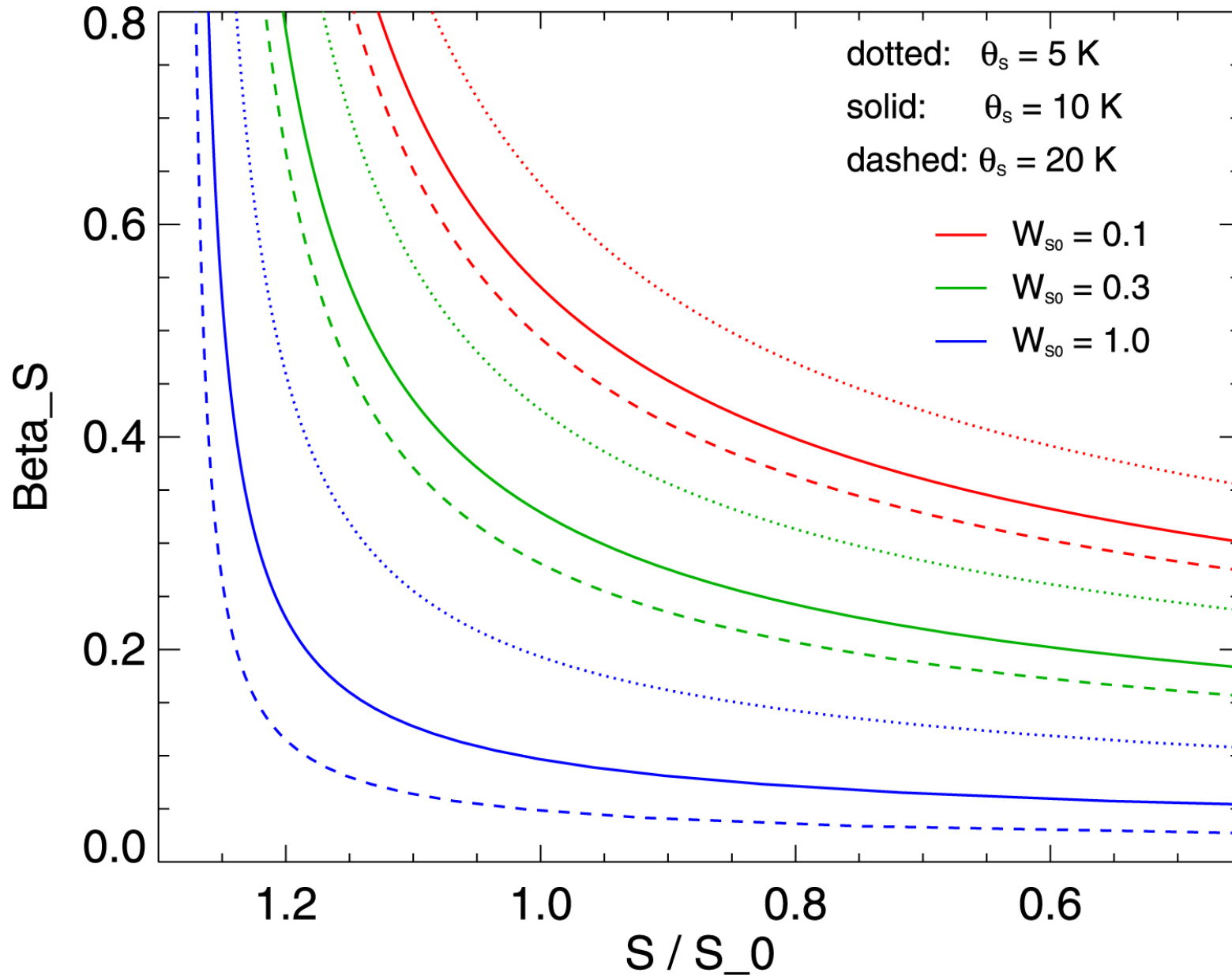
Figure 16. from The Effect of Seafloor Weathering on Planetary Habitability null 2020 APJ 896 96 doi:10.3847/1538-4357/ab94a4 https://dx.doi.org/10.3847/1538-4357/ab94a4 © 2020. The American Astronomical Society. All rights reserved.
