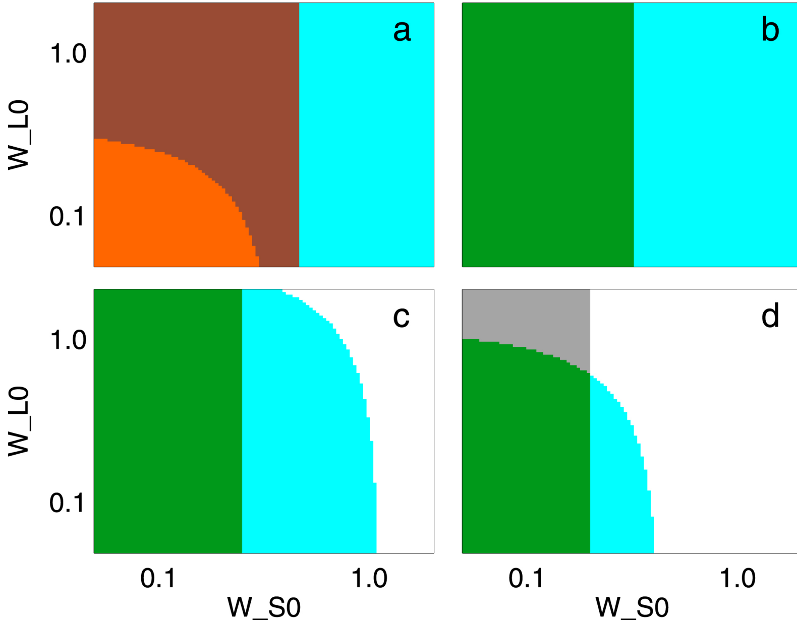
Figure 14. from The Effect of Seafloor Weathering on Planetary Habitability null 2020 APJ 896 96 doi:10.3847/1538-4357/ab94a4 https://dx.doi.org/10.3847/1538-4357/ab94a4 © 2020. The American Astronomical Society. All rights reserved.
