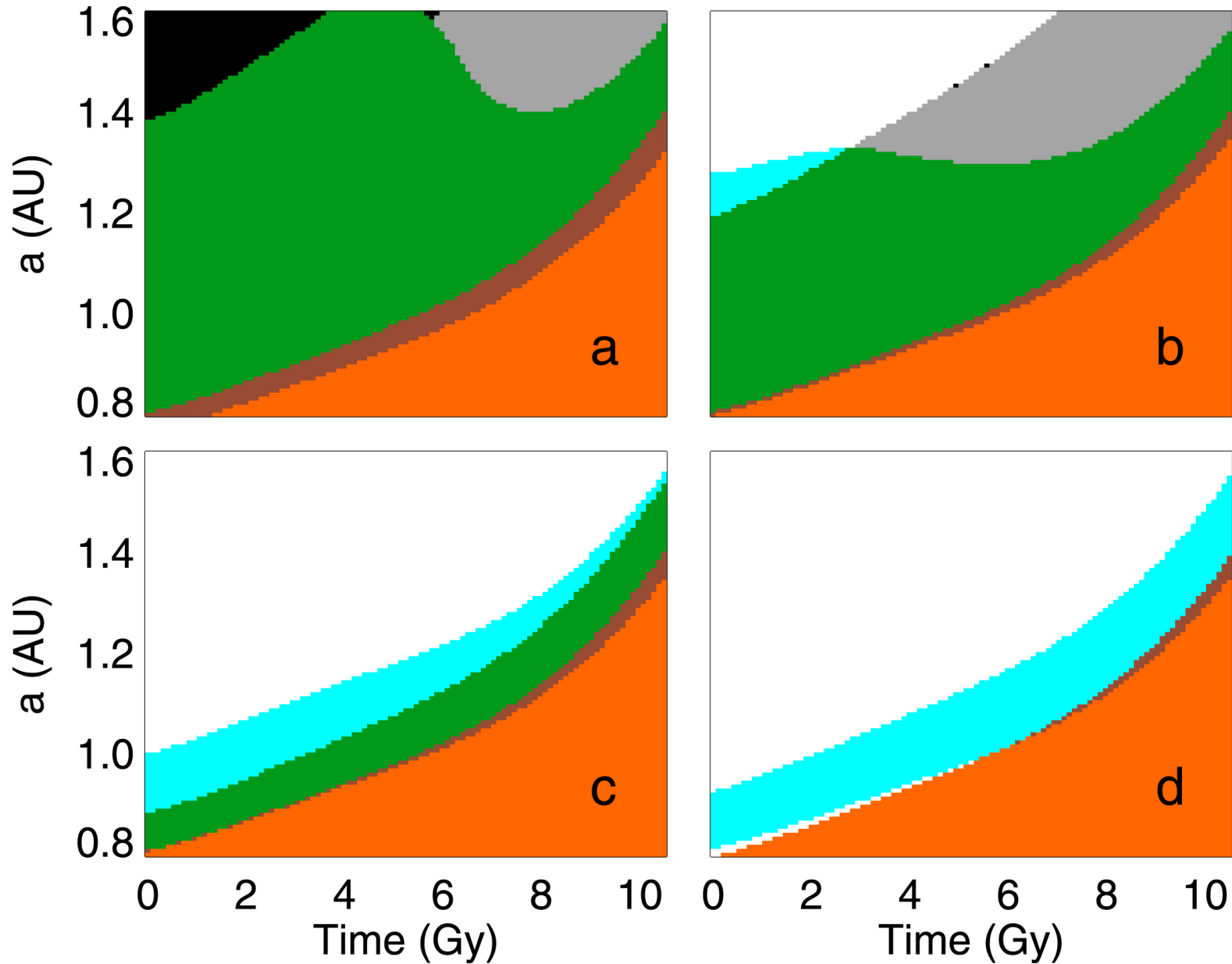
Figure 11. from The Effect of Seafloor Weathering on Planetary Habitability null 2020 APJ 896 96 doi:10.3847/1538-4357/ab94a4 https://dx.doi.org/10.3847/1538-4357/ab94a4 © 2020. The American Astronomical Society. All rights reserved.
