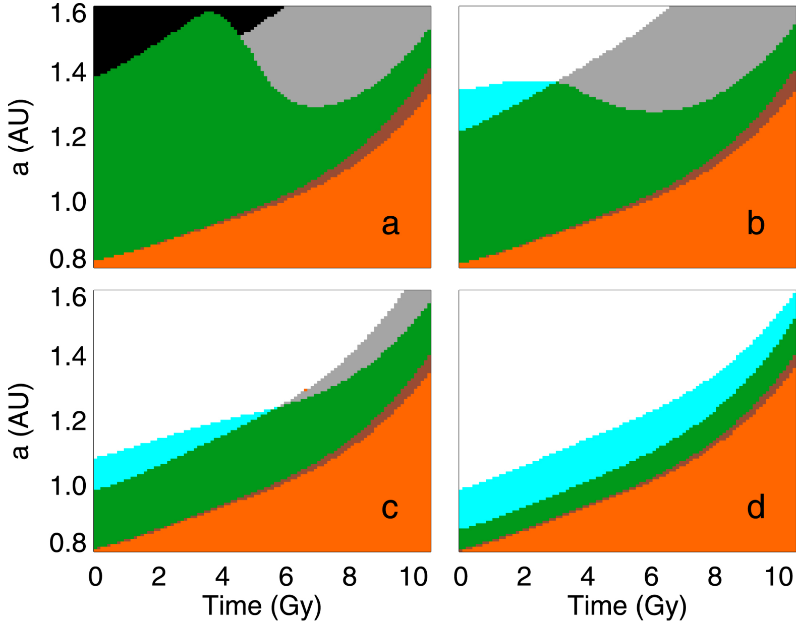
Figure 10. from The Effect of Seafloor Weathering on Planetary Habitability null 2020 APJ 896 96 doi:10.3847/1538-4357/ab94a4 https://dx.doi.org/10.3847/1538-4357/ab94a4 © 2020. The American Astronomical Society. All rights reserved.
