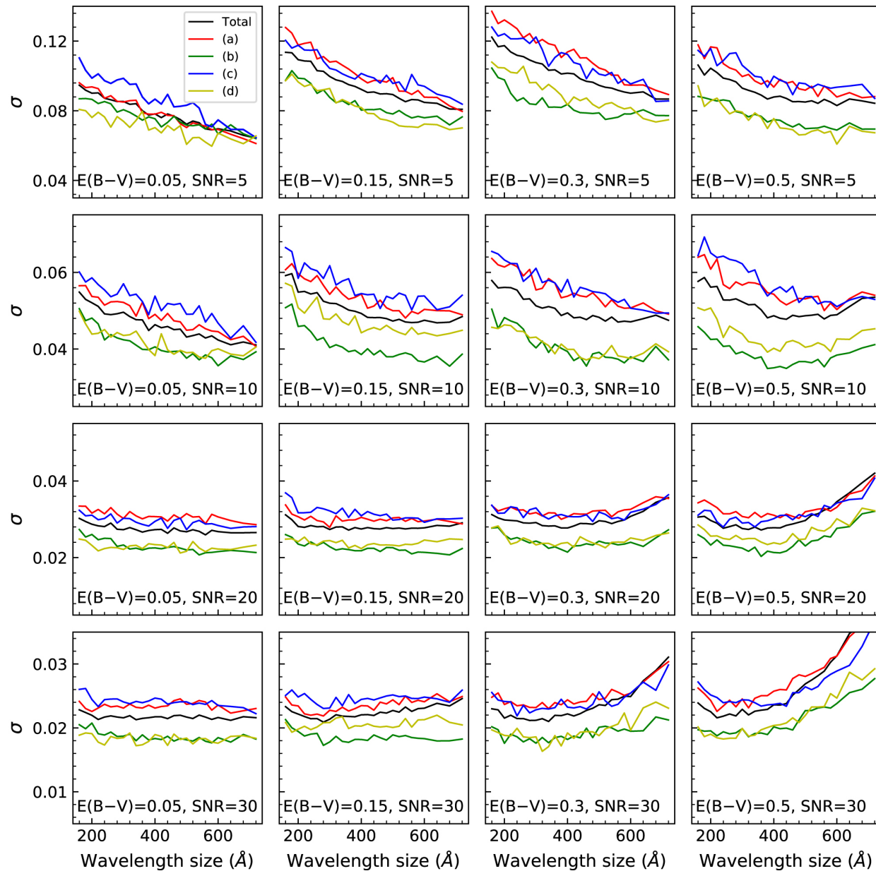
Figure 6. from Estimating Dust Attenuation from Galactic Spectra. I. Methodology and Tests null 2020 APJ 896 38 doi:10.3847/1538-4357/ab92a1 https://dx.doi.org/10.3847/1538-4357/ab92a1
