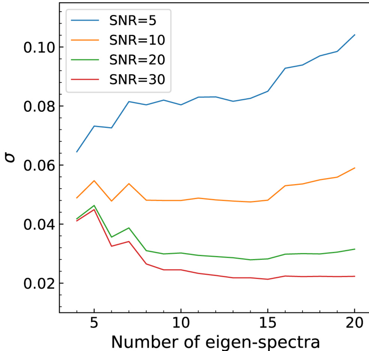
Figure 5. from Estimating Dust Attenuation from Galactic Spectra. I. Methodology and Tests null 2020 APJ 896 38 doi:10.3847/1538-4357/ab92a1 https://dx.doi.org/10.3847/1538-4357/ab92a1 © 2020. The Author(s). Published by the American Astronomical Society.
