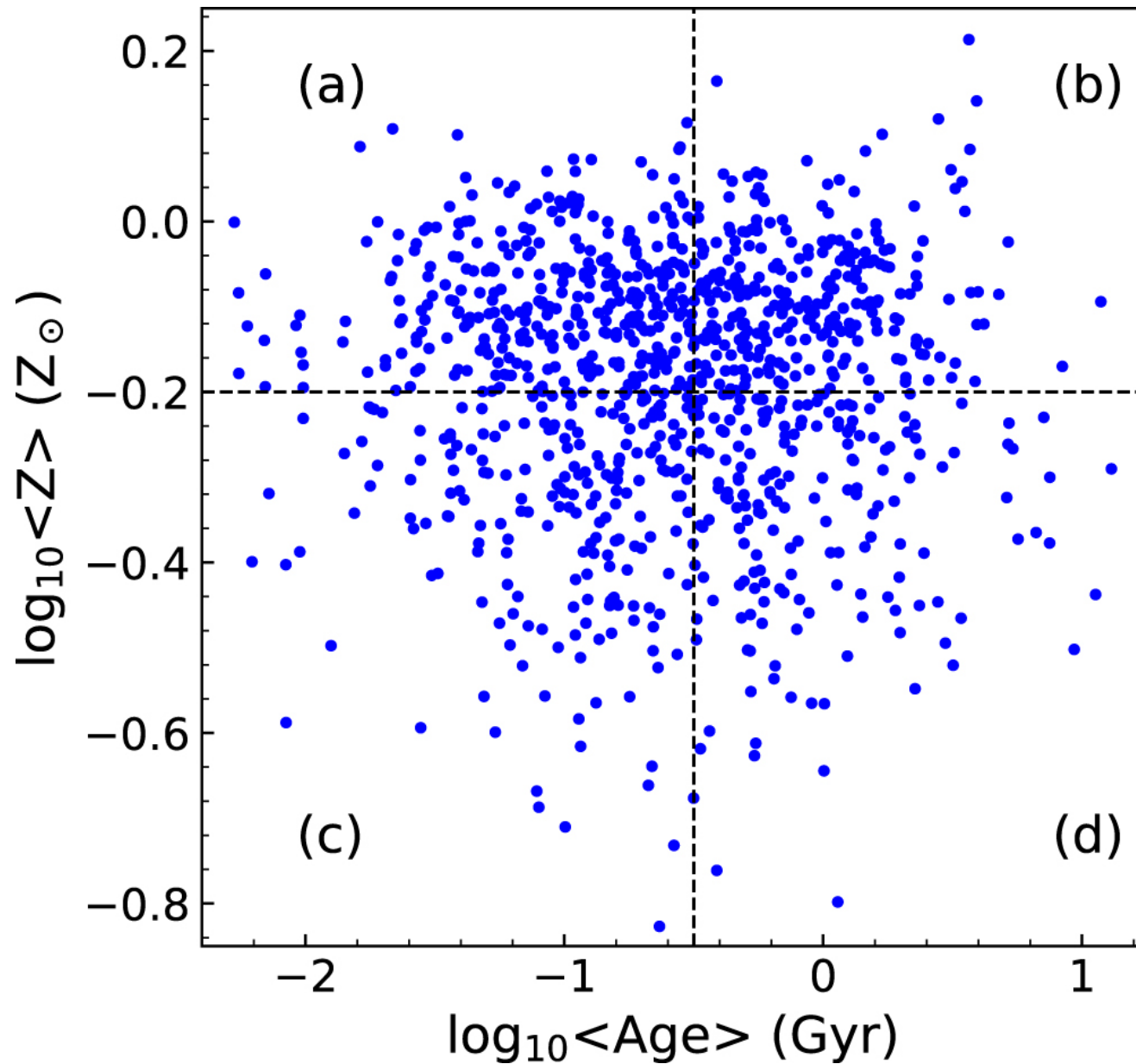
Figure 4. from Estimating Dust Attenuation from Galactic Spectra. I. Methodology and Tests null 2020 APJ 896 38 doi:10.3847/1538-4357/ab92a1 https://dx.doi.org/10.3847/1538-4357/ab92a1 © 2020. The Author(s). Published by the American Astronomical Society.
