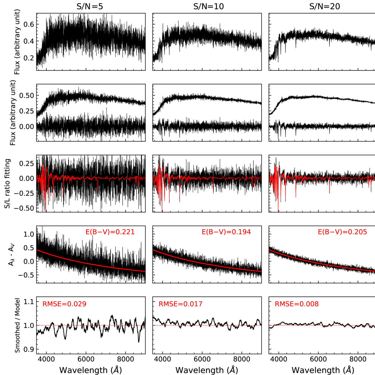
Figure 3. from Estimating Dust Attenuation from Galactic Spectra. I. Methodology and Tests null 2020 APJ 896 38 doi:10.3847/1538-4357/ab92a1 https://dx.doi.org/10.3847/1538-4357/ab92a1
