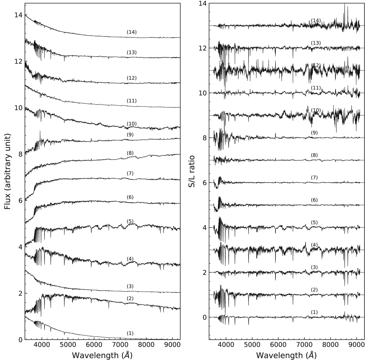
Figure 2. from Estimating Dust Attenuation from Galactic Spectra. I. Methodology and Tests null 2020 APJ 896 38 doi:10.3847/1538-4357/ab92a1 https://dx.doi.org/10.3847/1538-4357/ab92a1 © 2020. The Author(s). Published by the American Astronomical Society.
