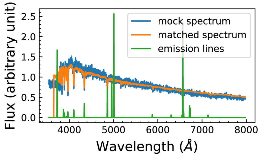
Figure A1. from Estimating Dust Attenuation from Galactic Spectra. I. Methodology and Tests null 2020 APJ 896 38 doi:10.3847/1538-4357/ab92a1 https://dx.doi.org/10.3847/1538-4357/ab92a1 © 2020. The Author(s). Published by the American Astronomical Society.
