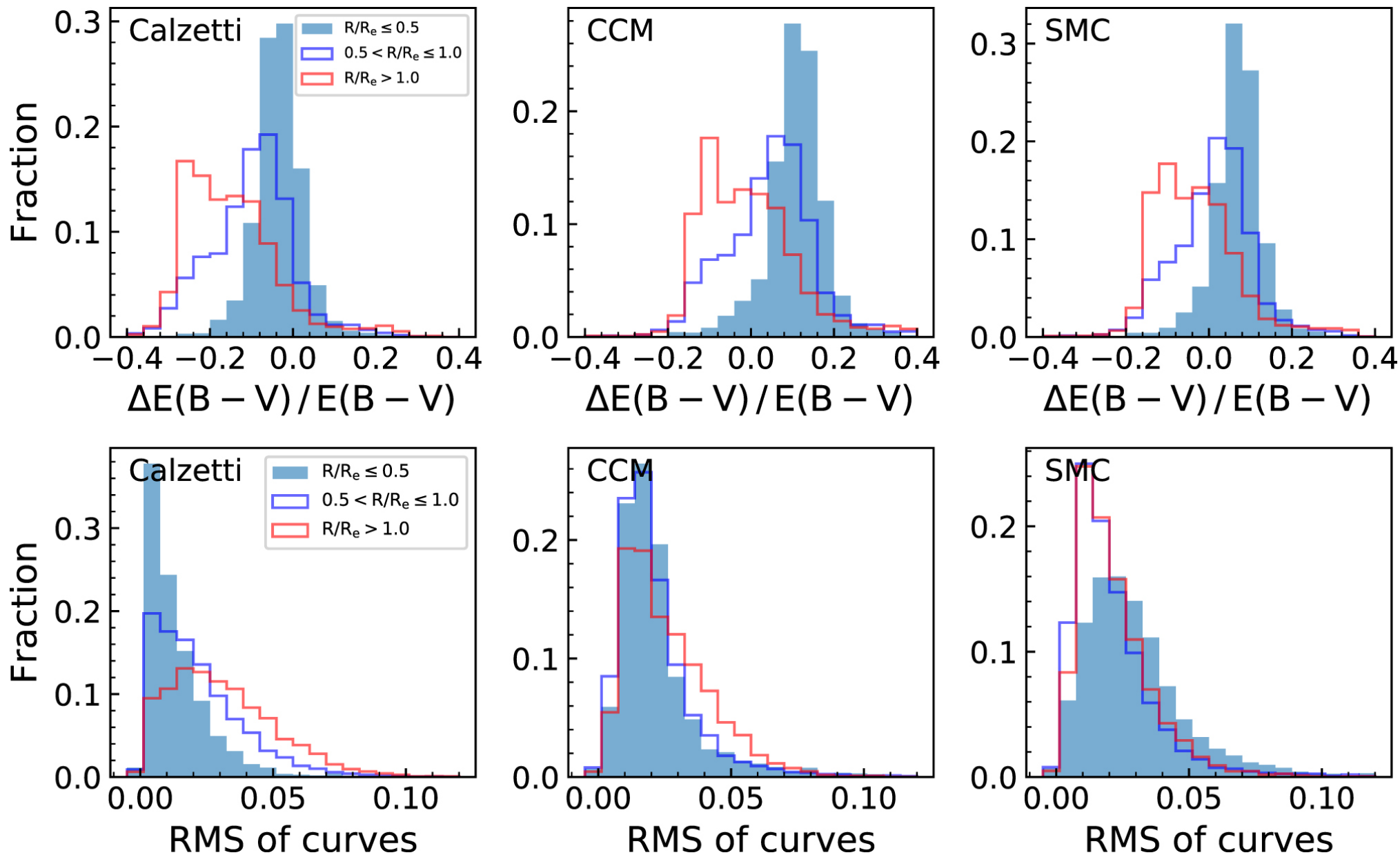
Figure 12. from Estimating Dust Attenuation from Galactic Spectra. I. Methodology and Tests null 2020 APJ 896 38 doi:10.3847/1538-4357/ab92a1 https://dx.doi.org/10.3847/1538-4357/ab92a1
