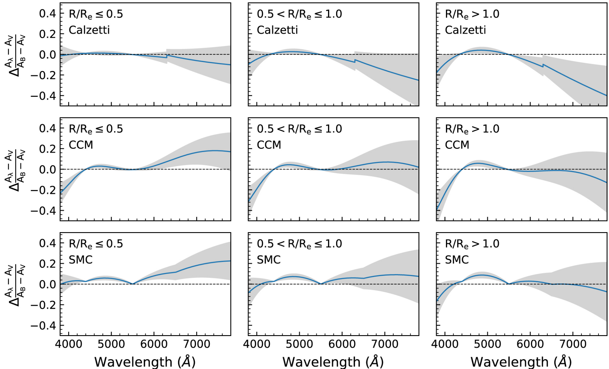
Figure 11. from Estimating Dust Attenuation from Galactic Spectra. I. Methodology and Tests null 2020 APJ 896 38 doi:10.3847/1538-4357/ab92a1 https://dx.doi.org/10.3847/1538-4357/ab92a1 © 2020. The Author(s). Published by the American Astronomical Society.
