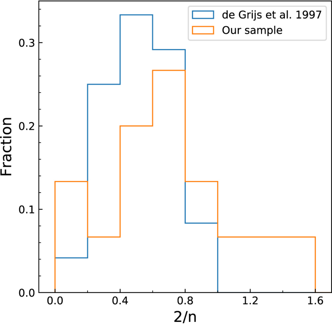
Figure 10. from Estimating Dust Attenuation from Galactic Spectra. I. Methodology and Tests null 2020 APJ 896 38 doi:10.3847/1538-4357/ab92a1 https://dx.doi.org/10.3847/1538-4357/ab92a1 © 2020. The Author(s). Published by the American Astronomical Society.
