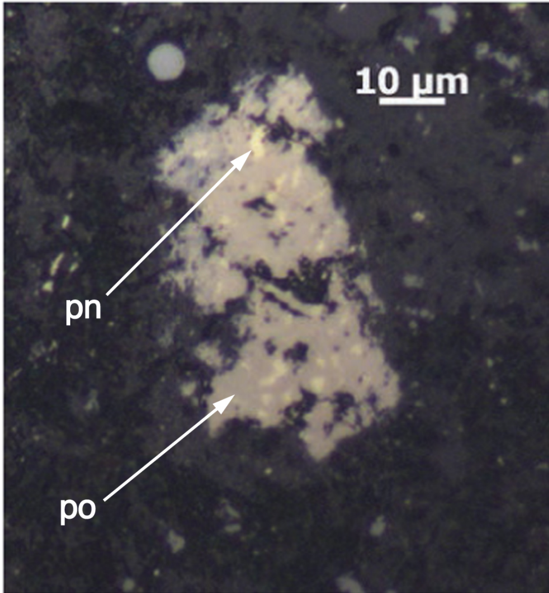
Figure 9. from Constraints on the Distances and Timescales of Solid Migration in the Early Solar System from Meteorite Magnetism null 2020 APJ 896 103 doi:10.3847/1538-4357/ab91ab https://dx.doi.org/10.3847/1538-4357/ab91ab © 2020. The American Astronomical Society. All rights reserved.
