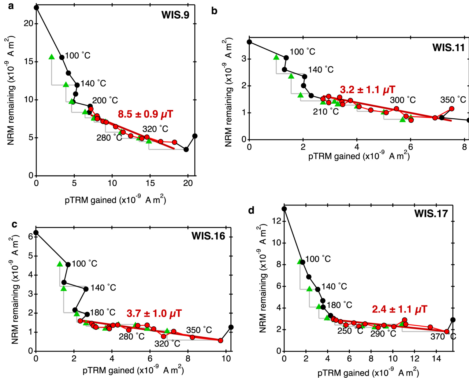
Figure 8. from Constraints on the Distances and Timescales of Solid Migration in the Early Solar System from Meteorite Magnetism null 2020 APJ 896 103 doi:10.3847/1538-4357/ab91ab https://dx.doi.org/10.3847/1538-4357/ab91ab © 2020. The American Astronomical Society. All rights reserved.
