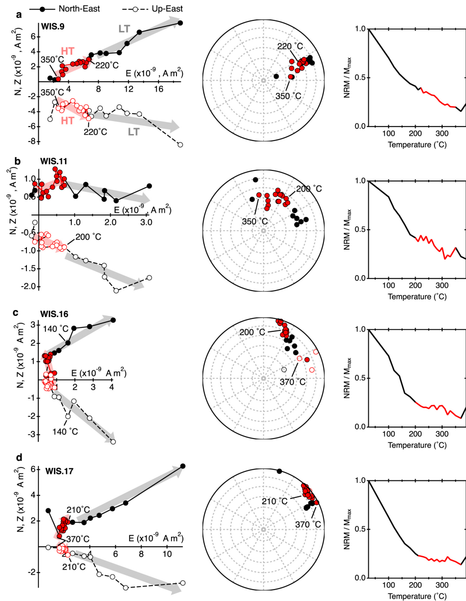
Figure 7. from Constraints on the Distances and Timescales of Solid Migration in the Early Solar System from Meteorite Magnetism null 2020 APJ 896 103 doi:10.3847/1538-4357/ab91ab https://dx.doi.org/10.3847/1538-4357/ab91ab © 2020. The American Astronomical Society. All rights reserved.
