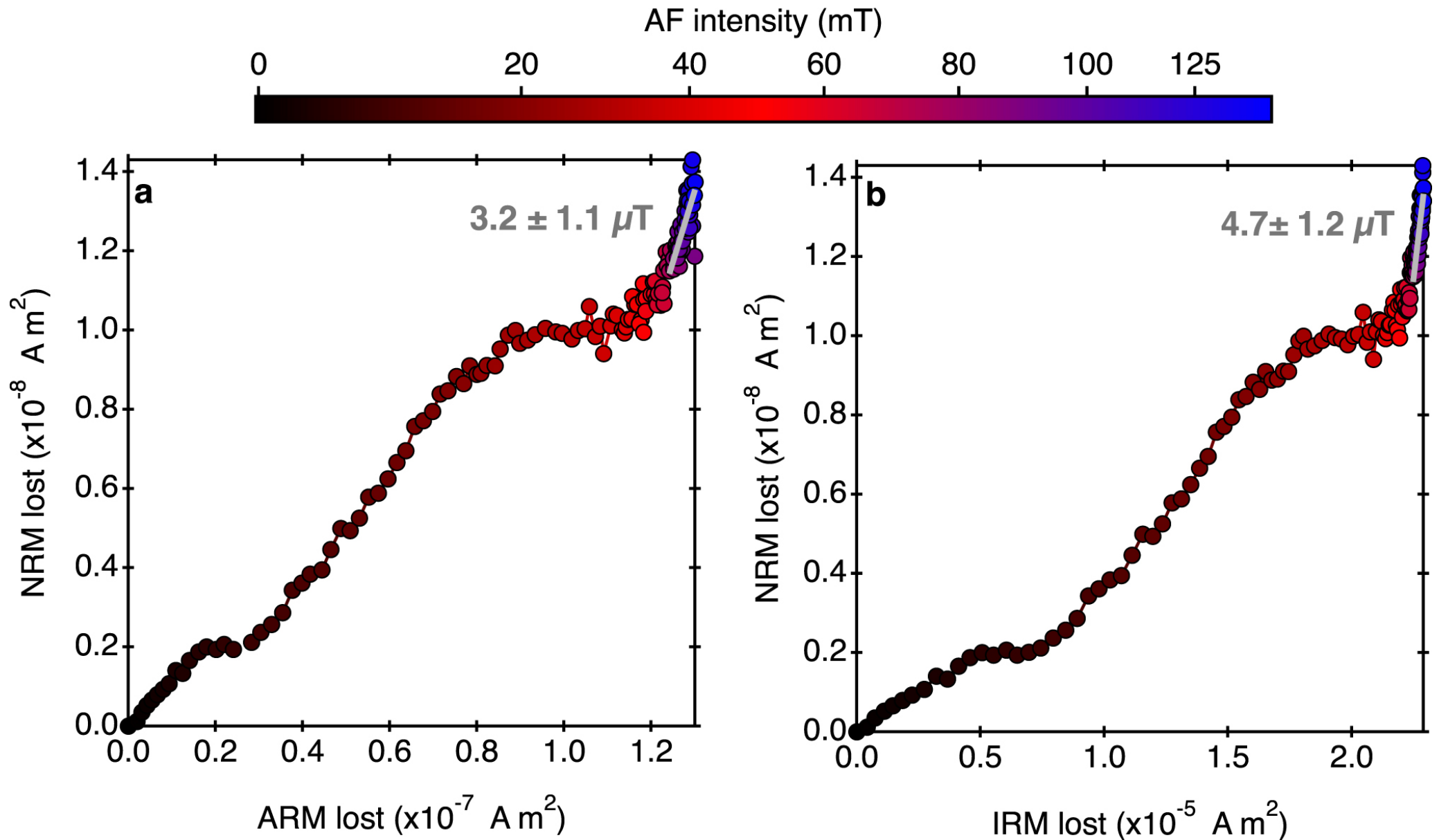
Figure 6. from Constraints on the Distances and Timescales of Solid Migration in the Early Solar System from Meteorite Magnetism null 2020 APJ 896 103 doi:10.3847/1538-4357/ab91ab https://dx.doi.org/10.3847/1538-4357/ab91ab © 2020. The American Astronomical Society. All rights reserved.
