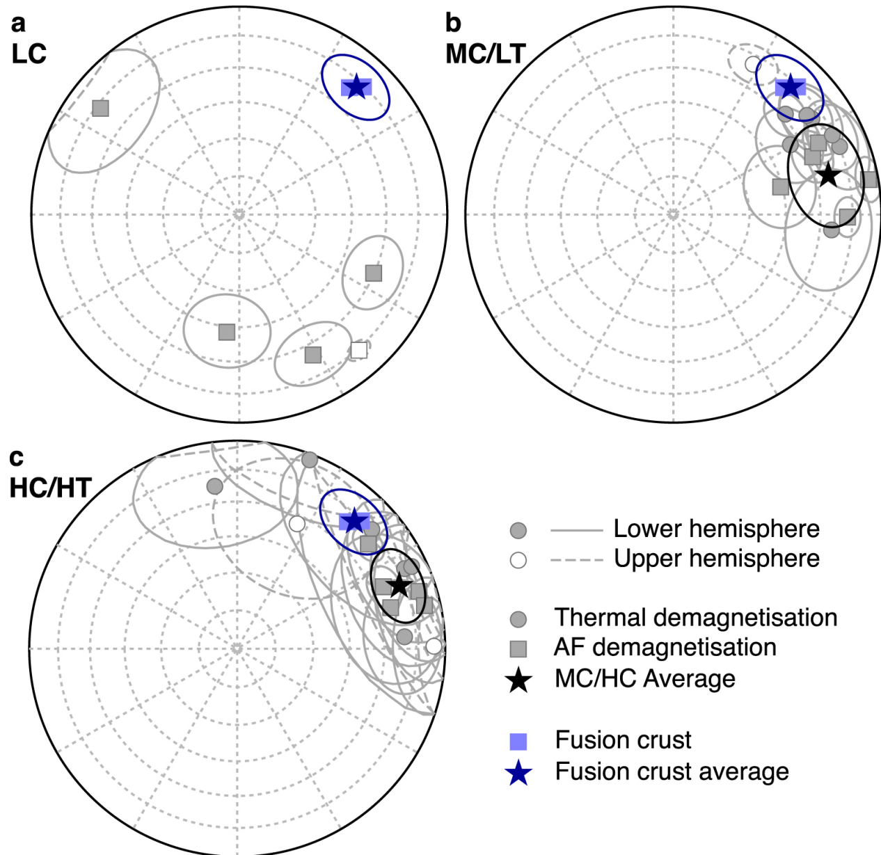
Figure 5. from Constraints on the Distances and Timescales of Solid Migration in the Early Solar System from Meteorite Magnetism null 2020 APJ 896 103 doi:10.3847/1538-4357/ab91ab https://dx.doi.org/10.3847/1538-4357/ab91ab © 2020. The American Astronomical Society. All rights reserved.
