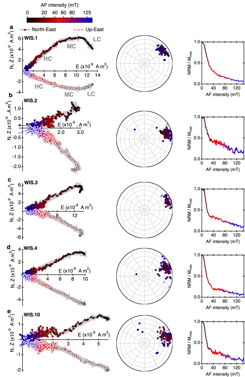
Figure 4. from Constraints on the Distances and Timescales of Solid Migration in the Early Solar System from Meteorite Magnetism null 2020 APJ 896 103 doi:10.3847/1538-4357/ab91ab https://dx.doi.org/10.3847/1538-4357/ab91ab © 2020. The American Astronomical Society. All rights reserved.
