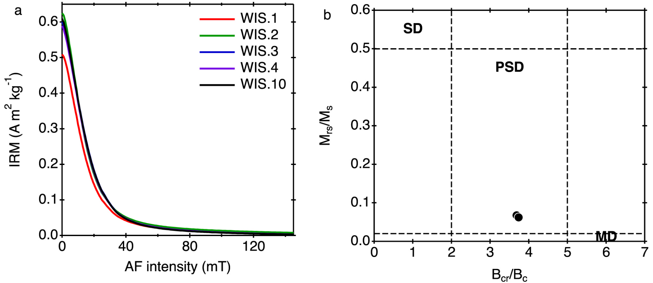
Figure 2. from Constraints on the Distances and Timescales of Solid Migration in the Early Solar System from Meteorite Magnetism null 2020 APJ 896 103 doi:10.3847/1538-4357/ab91ab https://dx.doi.org/10.3847/1538-4357/ab91ab © 2020. The American Astronomical Society. All rights reserved.
