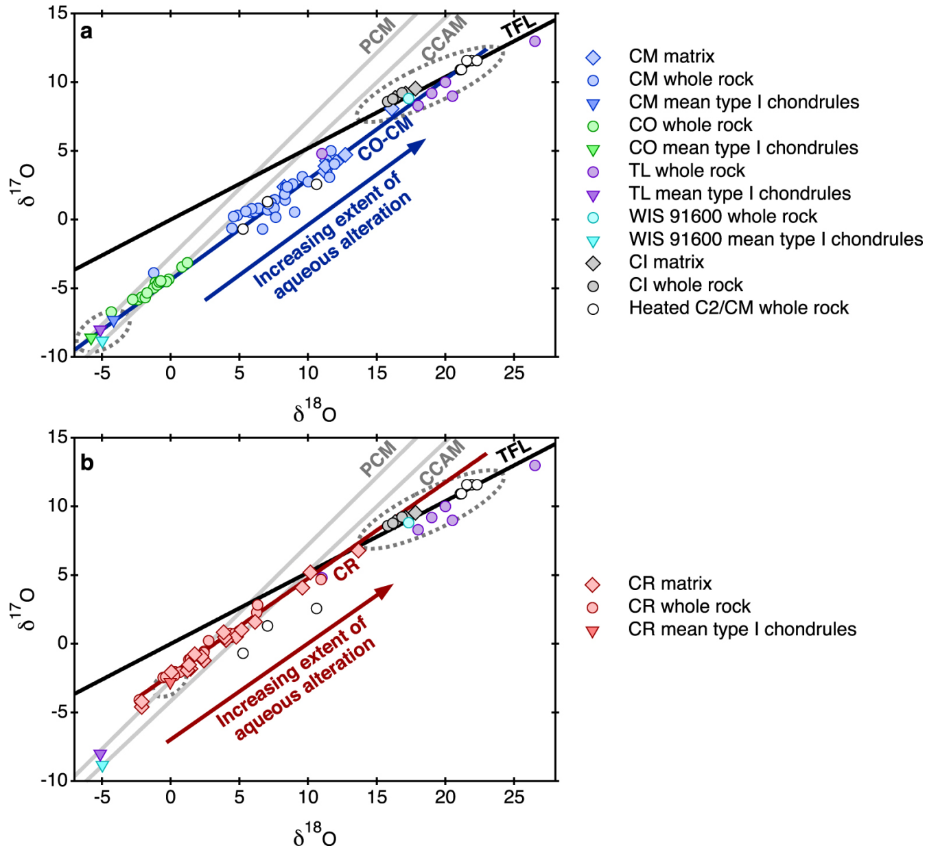
Figure 13. from Constraints on the Distances and Timescales of Solid Migration in the Early Solar System from Meteorite Magnetism null 2020 APJ 896 103 doi:10.3847/1538-4357/ab91ab https://dx.doi.org/10.3847/1538-4357/ab91ab
