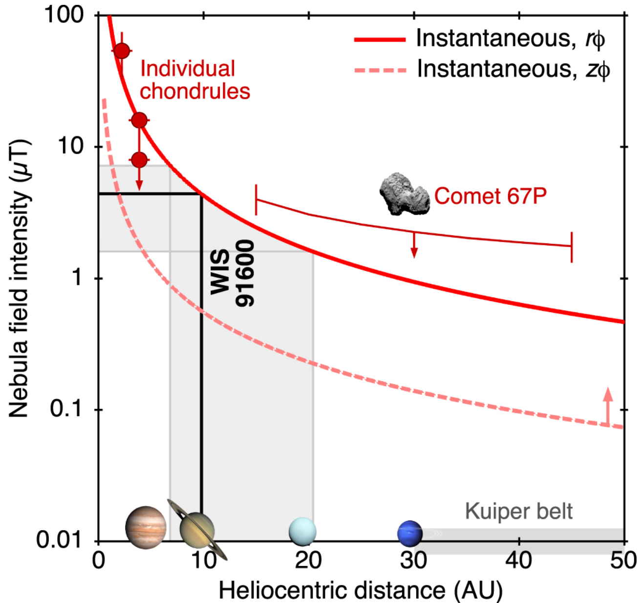
Figure 12. from Constraints on the Distances and Timescales of Solid Migration in the Early Solar System from Meteorite Magnetism null 2020 APJ 896 103 doi:10.3847/1538-4357/ab91ab https://dx.doi.org/10.3847/1538-4357/ab91ab © 2020. The American Astronomical Society. All rights reserved.
