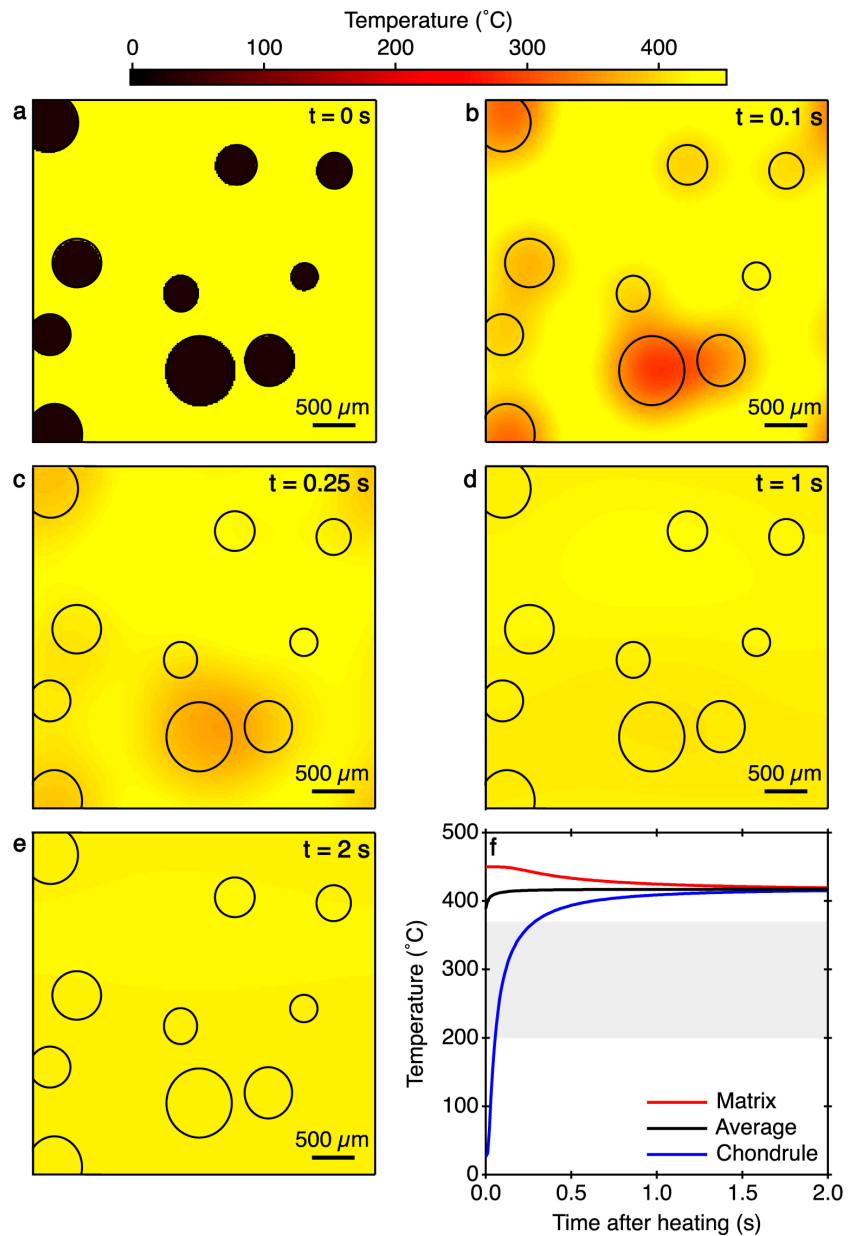
Figure 10. from Constraints on the Distances and Timescales of Solid Migration in the Early Solar System from Meteorite Magnetism null 2020 APJ 896 103 doi:10.3847/1538-4357/ab91ab https://dx.doi.org/10.3847/1538-4357/ab91ab © 2020. The American Astronomical Society. All rights reserved.
