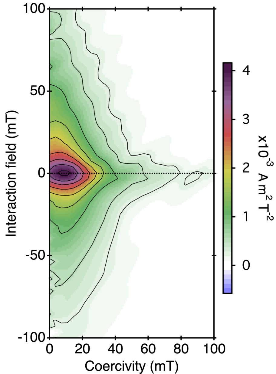
Figure 1. from Constraints on the Distances and Timescales of Solid Migration in the Early Solar System from Meteorite Magnetism null 2020 APJ 896 103 doi:10.3847/1538-4357/ab91ab https://dx.doi.org/10.3847/1538-4357/ab91ab © 2020. The American Astronomical Society. All rights reserved.
