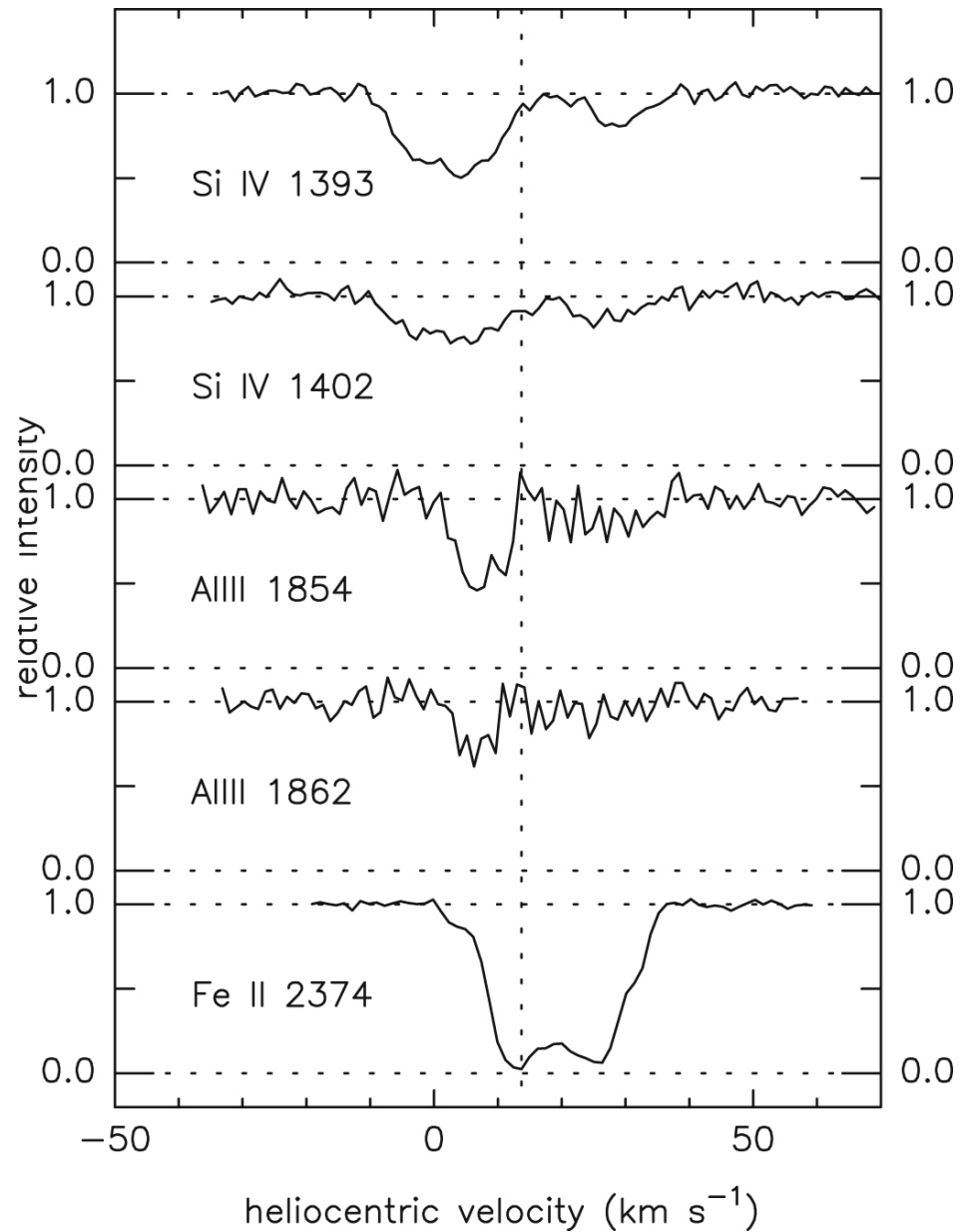
Figure 9. from HD 62542: Probing the Bare, Dense Core of a Translucent Interstellar Cloud null 2020 APJ 897 36 doi:10.3847/1538-4357/ab8f8e https://dx.doi.org/10.3847/1538-4357/ab8f8e © 2020. The American Astronomical Society. All rights reserved.
