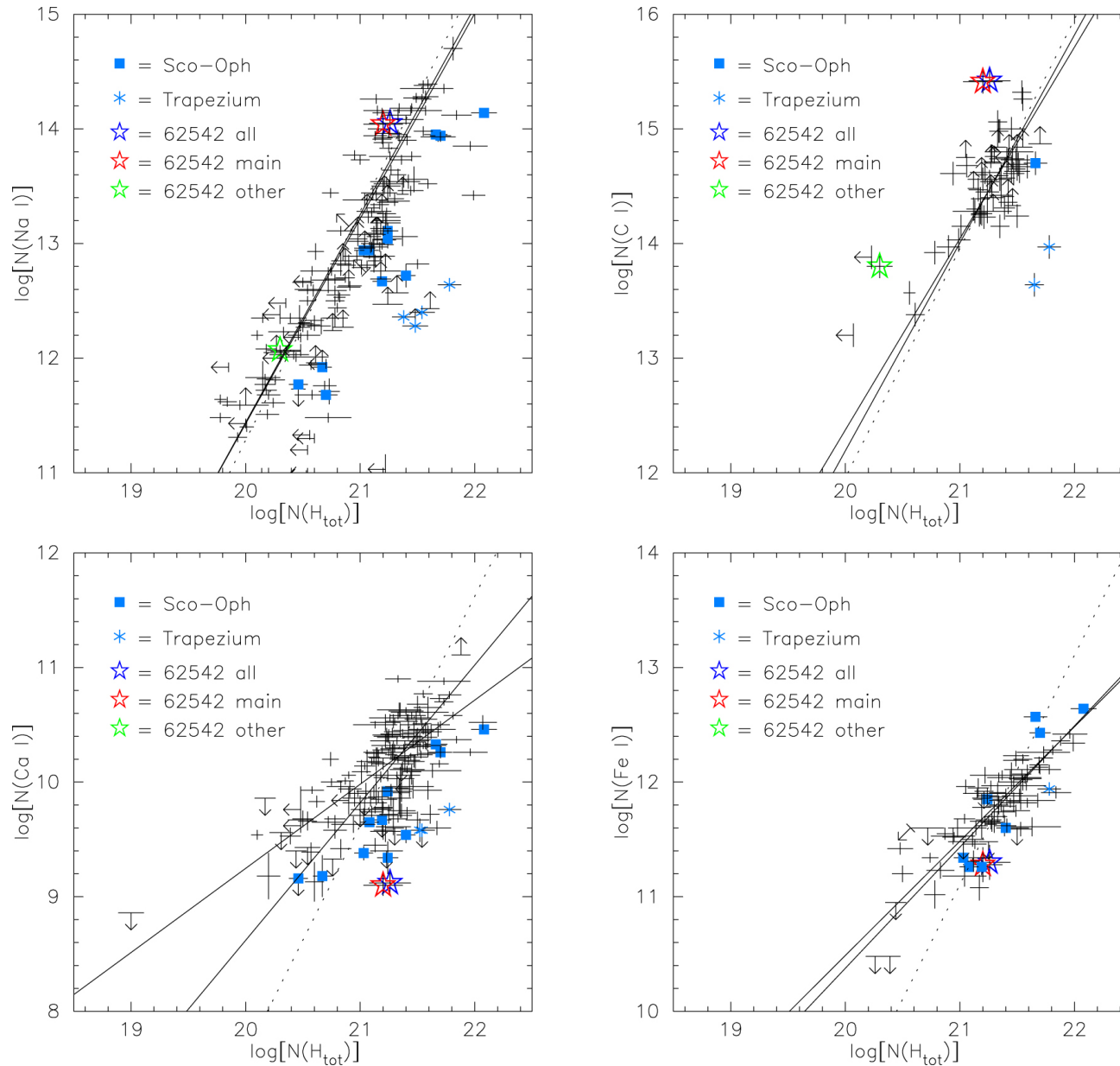
Figure 8. from HD 62542: Probing the Bare, Dense Core of a Translucent Interstellar Cloud null 2020 APJ 897 36 doi:10.3847/1538-4357/ab8f8e https://dx.doi.org/10.3847/1538-4357/ab8f8e
