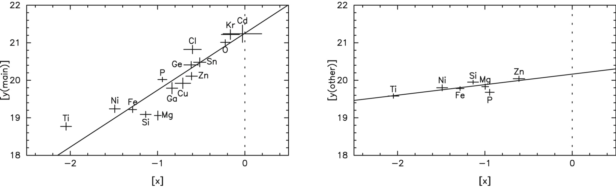
Figure 6. from HD 62542: Probing the Bare, Dense Core of a Translucent Interstellar Cloud null 2020 APJ 897 36 doi:10.3847/1538-4357/ab8f8e https://dx.doi.org/10.3847/1538-4357/ab8f8e © 2020. The American Astronomical Society. All rights reserved.
