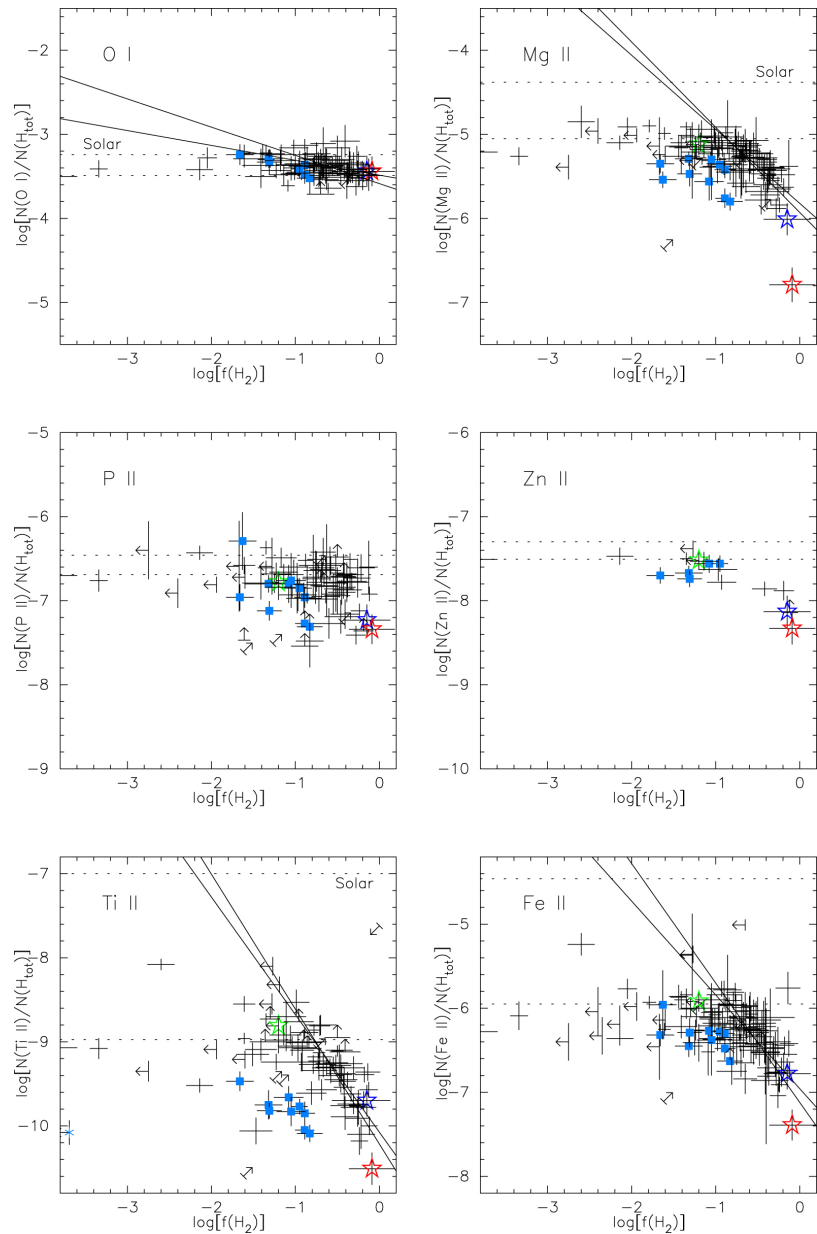
Figure 21. from HD 62542: Probing the Bare, Dense Core of a Translucent Interstellar Cloud null 2020 APJ 897 36 doi:10.3847/1538-4357/ab8f8e https://dx.doi.org/10.3847/1538-4357/ab8f8e © 2020. The American Astronomical Society. All rights reserved.
