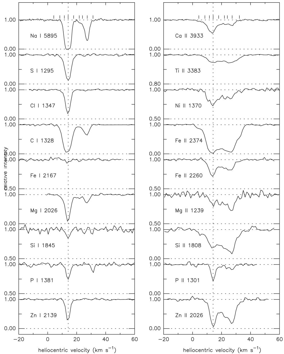
Figure 2. from HD 62542: Probing the Bare, Dense Core of a Translucent Interstellar Cloud null 2020 APJ 897 36 doi:10.3847/1538-4357/ab8f8e https://dx.doi.org/10.3847/1538-4357/ab8f8e © 2020. The American Astronomical Society. All rights reserved.
