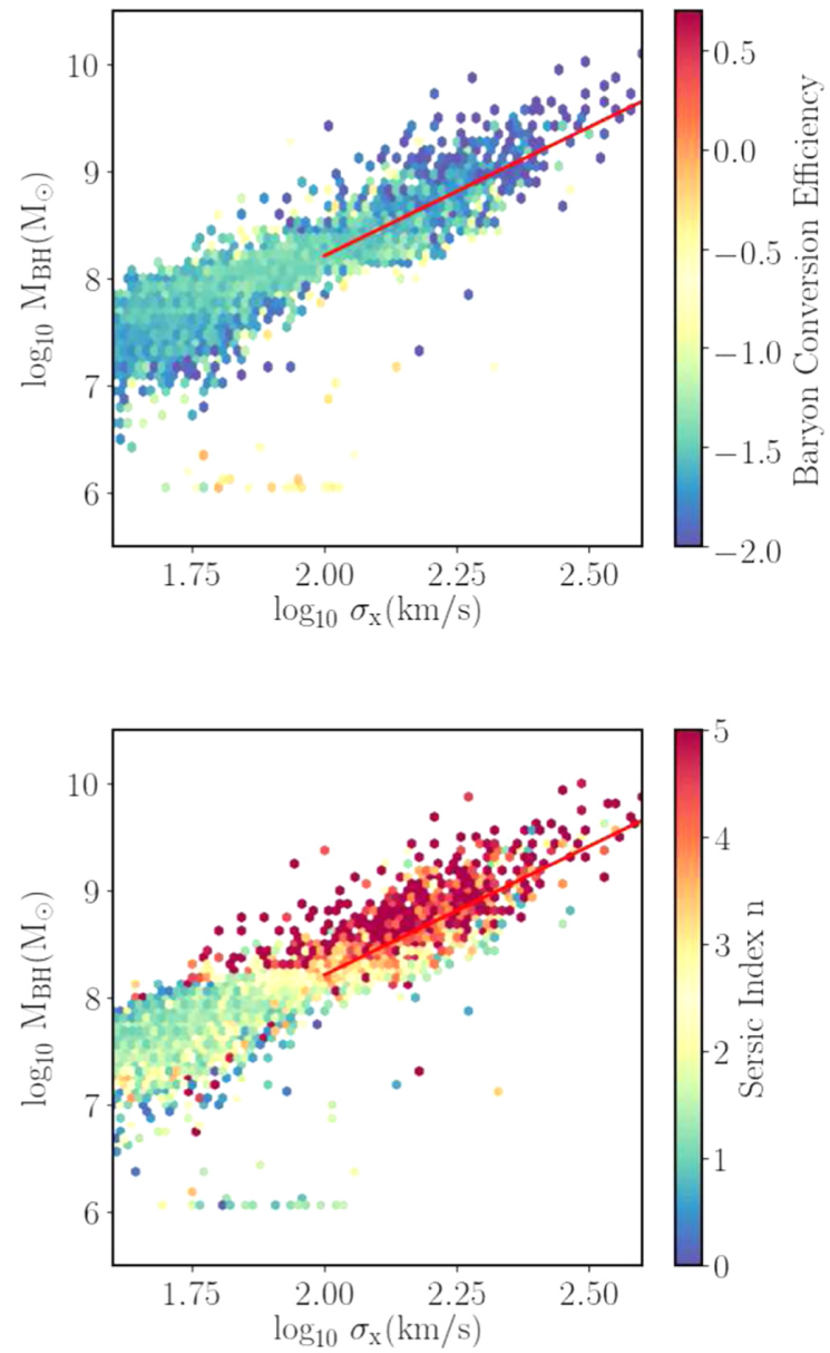
Figure 9. from Correlations between Black Holes and Host Galaxies in the Illustris and IllustrisTNG Simulations null 2020 APJ 895 102 doi:10.3847/1538-4357/ab8f8d https://dx.doi.org/10.3847/1538-4357/ab8f8d © 2020. The American Astronomical Society. All rights reserved.
