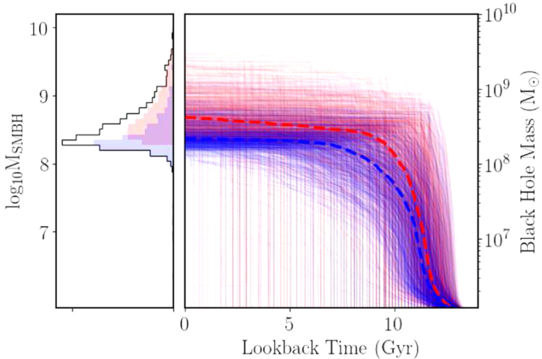
Figure 8. from Correlations between Black Holes and Host Galaxies in the Illustris and IllustrisTNG Simulations null 2020 APJ 895 102 doi:10.3847/1538-4357/ab8f8d https://dx.doi.org/10.3847/1538-4357/ab8f8d © 2020. The American Astronomical Society. All rights reserved.
