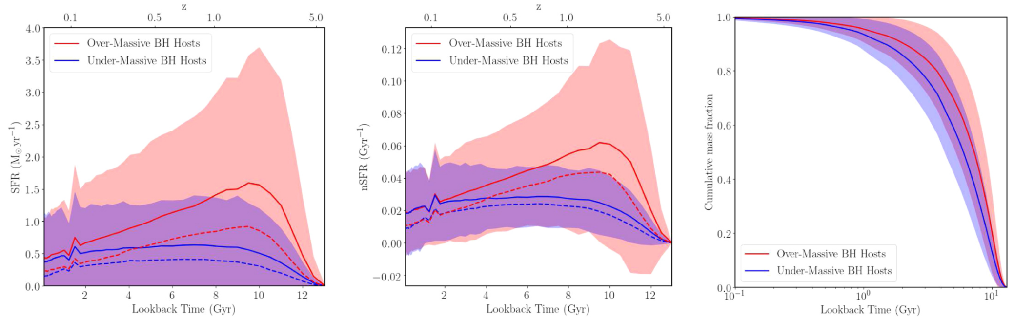
Figure 6. from Correlations between Black Holes and Host Galaxies in the Illustris and IllustrisTNG Simulations null 2020 APJ 895 102 doi:10.3847/1538-4357/ab8f8d https://dx.doi.org/10.3847/1538-4357/ab8f8d © 2020. The American Astronomical Society. All rights reserved.
