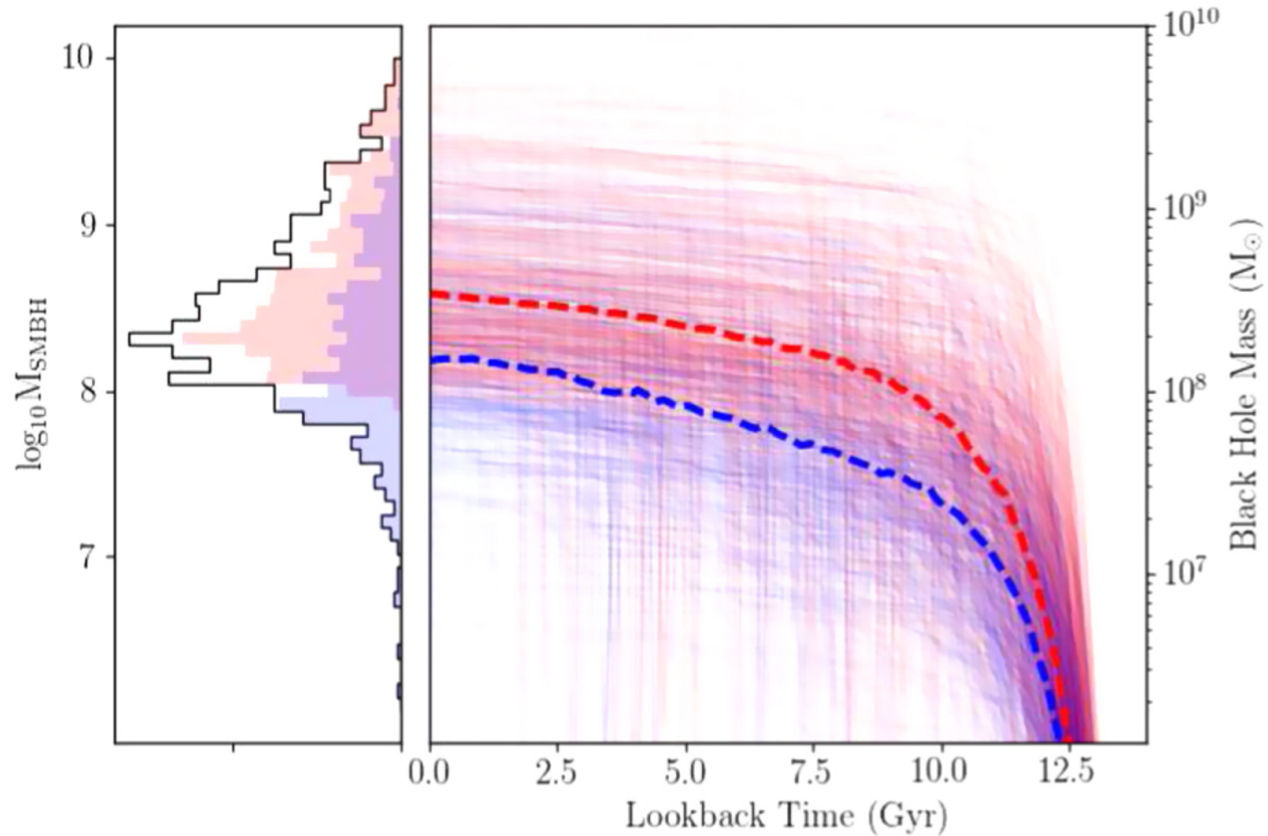
Figure 5. from Correlations between Black Holes and Host Galaxies in the Illustris and IllustrisTNG Simulations null 2020 APJ 895 102 doi:10.3847/1538-4357/ab8f8d https://dx.doi.org/10.3847/1538-4357/ab8f8d © 2020. The American Astronomical Society. All rights reserved.
