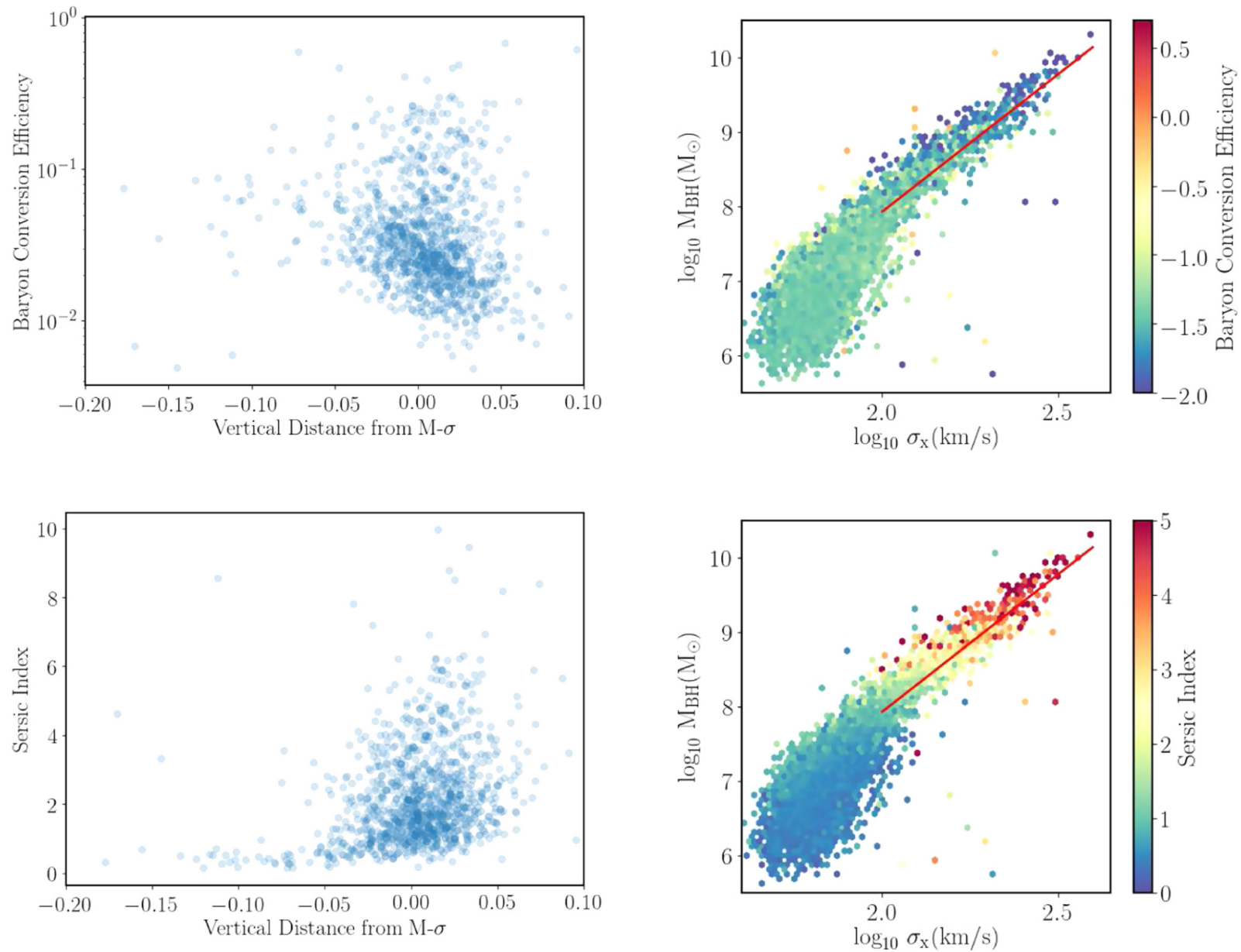
Figure 4. from Correlations between Black Holes and Host Galaxies in the Illustris and IllustrisTNG Simulations null 2020 APJ 895 102 doi:10.3847/1538-4357/ab8f8d https://dx.doi.org/10.3847/1538-4357/ab8f8d © 2020. The American Astronomical Society. All rights reserved.
