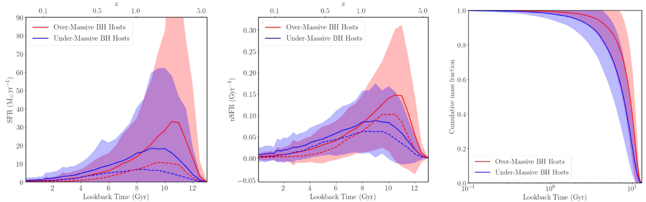
Figure 3. from Correlations between Black Holes and Host Galaxies in the Illustris and IllustrisTNG Simulations null 2020 APJ 895 102 doi:10.3847/1538-4357/ab8f8d https://dx.doi.org/10.3847/1538-4357/ab8f8d © 2020. The American Astronomical Society. All rights reserved.
