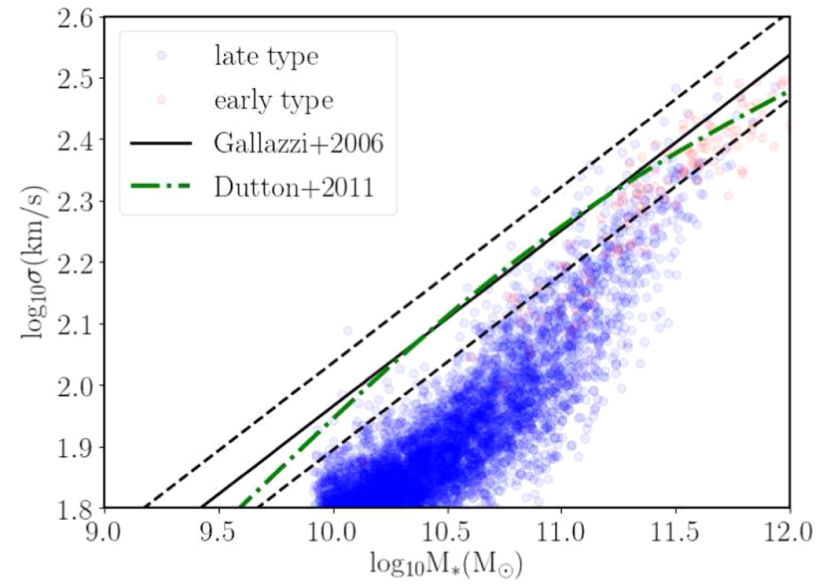
Figure 2. from Correlations between Black Holes and Host Galaxies in the Illustris and IllustrisTNG Simulations null 2020 APJ 895 102 doi:10.3847/1538-4357/ab8f8d https://dx.doi.org/10.3847/1538-4357/ab8f8d
