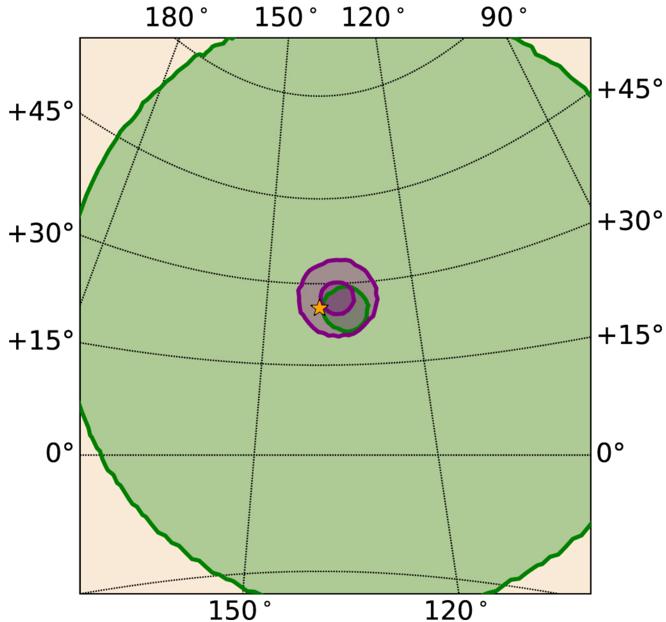
Figure 7. from Evaluation of Automated Fermi GBM Localizations of Gamma-Ray Bursts null 2020 APJ 895 40 doi:10.3847/1538-4357/ab8bdb https://dx.doi.org/10.3847/1538-4357/ab8bdb © 2020. The American Astronomical Society. All rights reserved.
